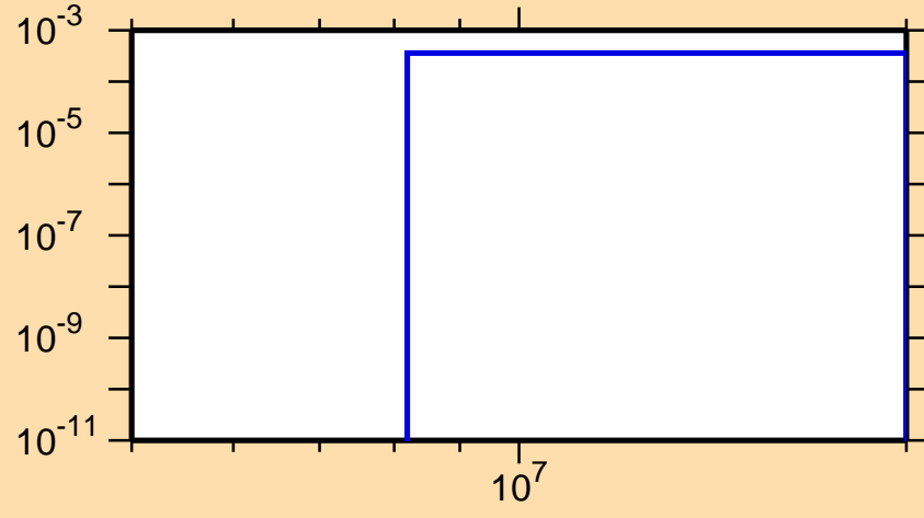
\sigma vs. E for ^{231}\text{U}(n,d)
