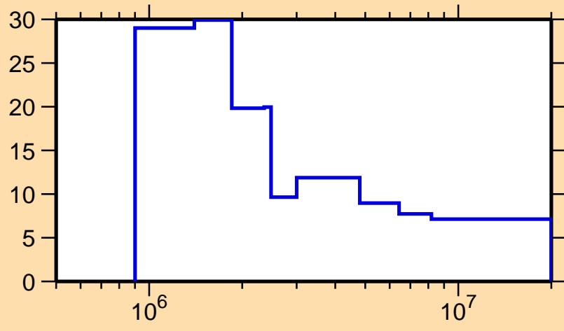
\Delta\sigma/\sigma vs. E for ^{231}\text{U}(n, nonel.)
