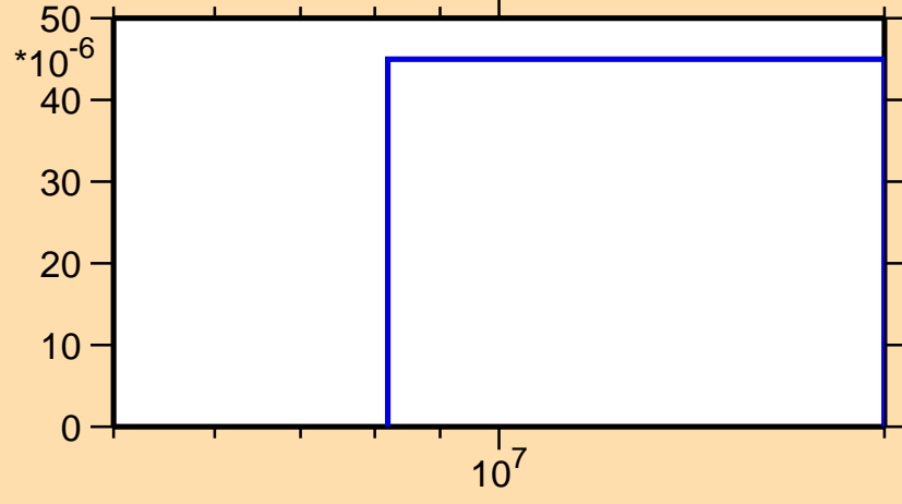
\sigma vs. E for ^{231}\text{U}(n,t)
