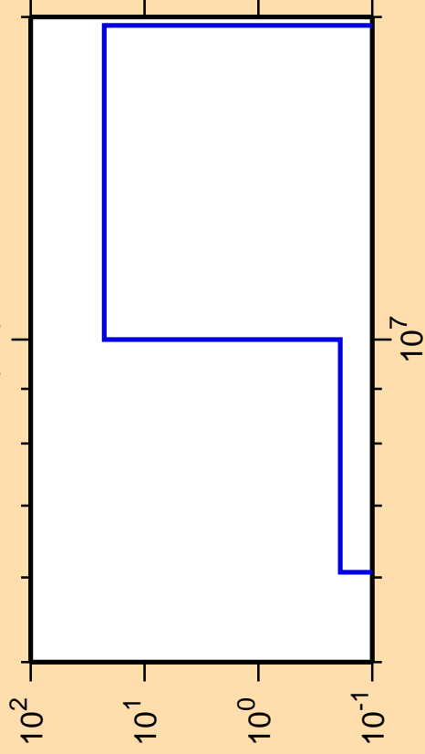
\Delta\sigma/\sigma vs. E for ^{235}\text{U}(n,t)
