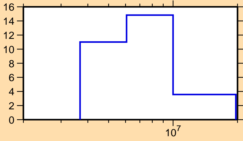
\Delta\sigma/\sigma vs. E for ^{235}\text{U}(n,el.)
