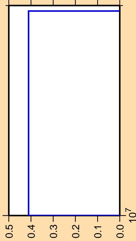
\Delta\sigma/\sigma vs. E for ^{235}\text{U}(n,\text{He3})
