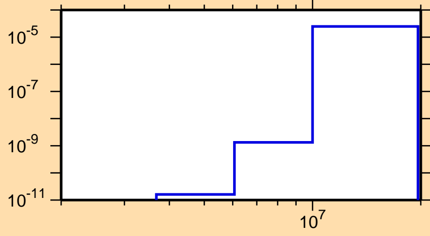
\sigma vs. E for ^{235}\text{U}(n,n\alpha)
