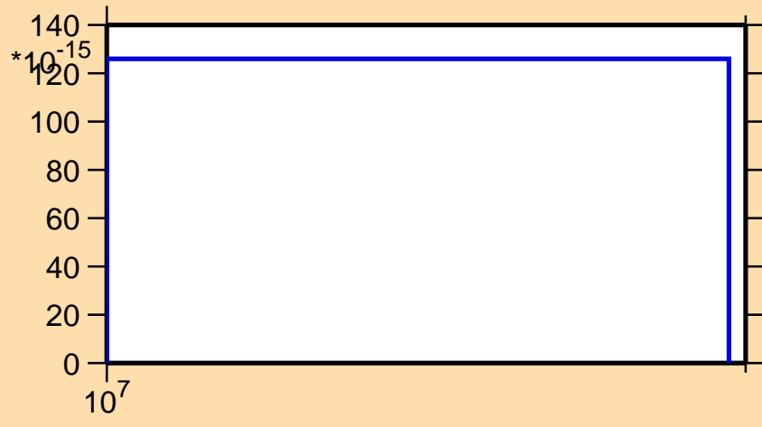
\sigma vs. E for ^{235}\text{U}(n,\text{He3})
