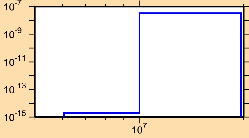
\sigma vs. E for ^{235}\text{U}(n,2n\alpha)
