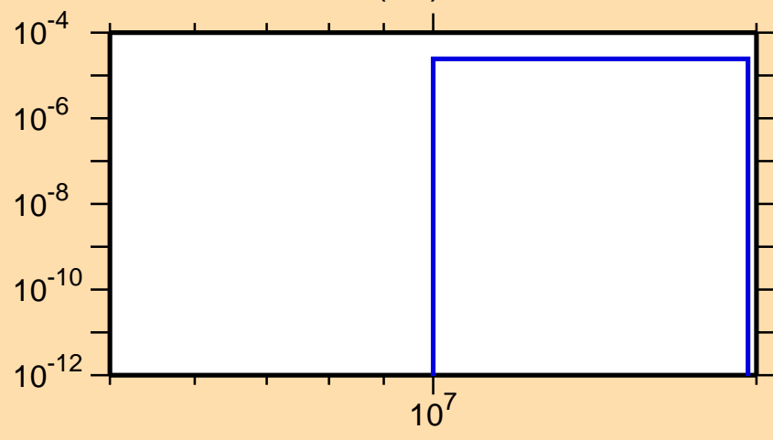
\sigma vs. E for ^{235}\text{U}(n,t)
