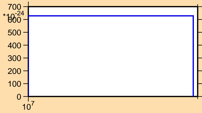
\sigma vs. E for ^{235}\text{U} (mt 42)
