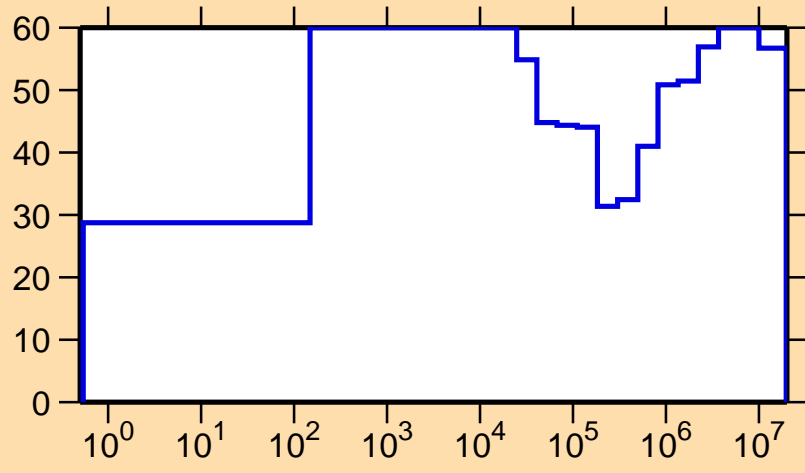
\Delta\sigma/\sigma vs. E for ^{235}\text{U}(n,f)
