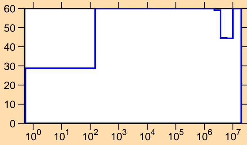
\Delta\sigma/\sigma vs. E for ^{235}\text{U}(n,\gamma)
