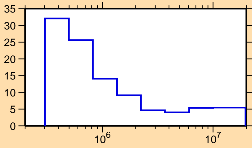
\Delta\sigma/\sigma vs. E for ^{235}\text{U}(n, nonel.)
