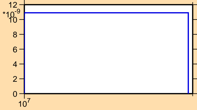
\sigma vs. E for ^{235}\text{U}(n,\text{nd})
