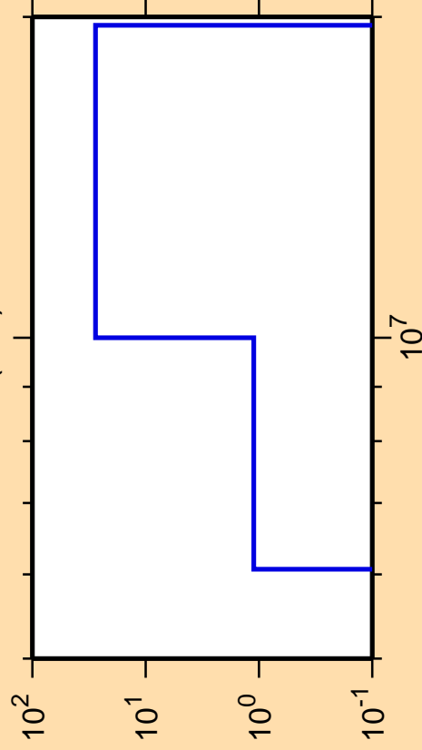
\Delta\sigma/\sigma vs. E for ^{235}\text{U}(n,d)
