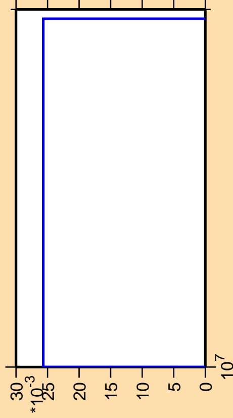
\Delta\sigma/\sigma vs. E for ^{235}\text{U}(n,3n\alpha)
