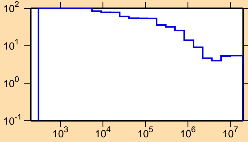
\Delta\sigma/\sigma vs. E for ^{235}\text{U}(n,\text{nonel.})
