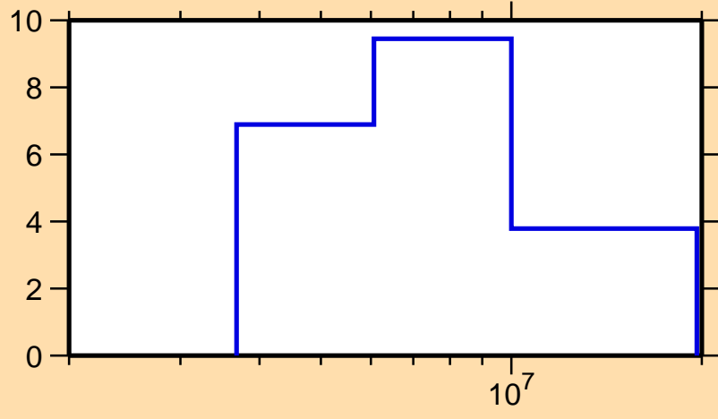
\Delta\sigma/\sigma vs. E for ^{235}\text{U}(n,\text{tot.})
