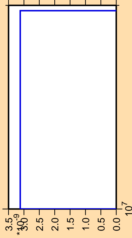
\Delta\sigma/\sigma vs. E for ^{235}\text{U} (mt 42)
