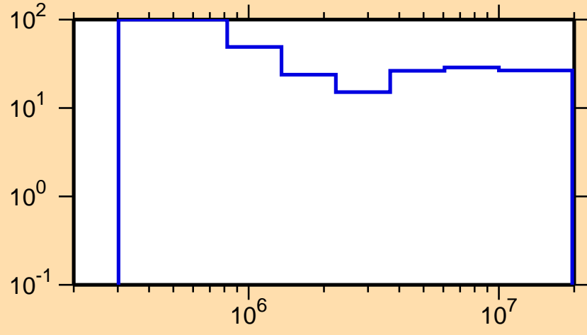
\Delta\sigma/\sigma vs. E for ^{235}\text{U}(n,n\text{cont.})
