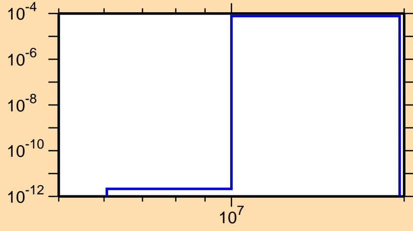
\sigma vs. E for ^{235}\text{U}(n,d)
