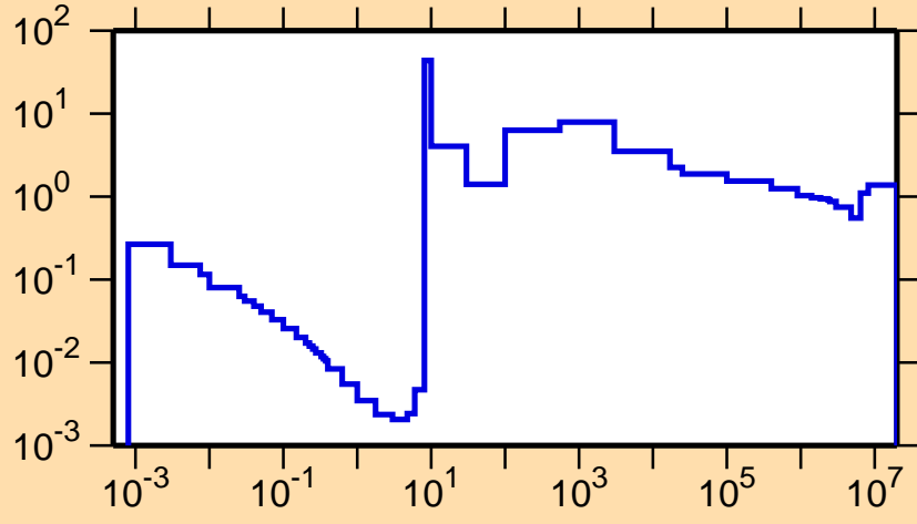
\sigma vs. E for ^{235}\text{U}(n,f)
