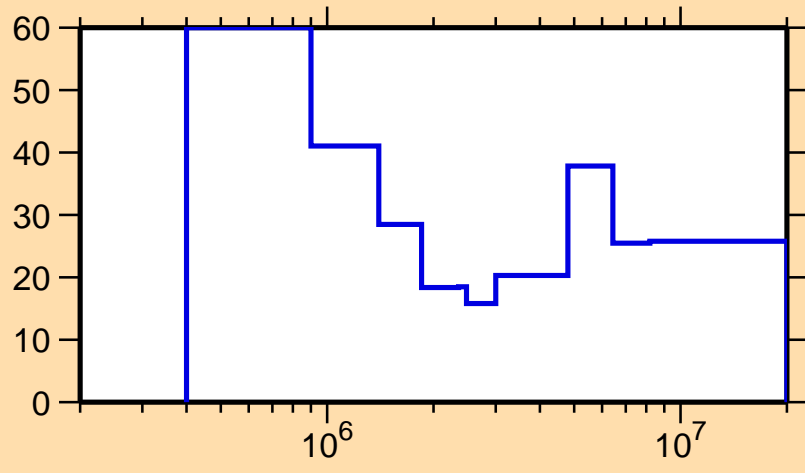
\Delta\sigma/\sigma vs. E for ^{235}\text{U}(n,n\text{cont.})
