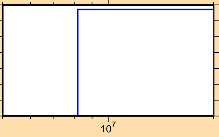
\sigma vs. E for ^{235}\text{U} (mt 42)
