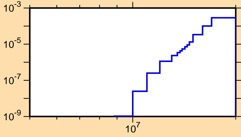
\sigma vs. E for ^{241}\text{U}(n,t)
