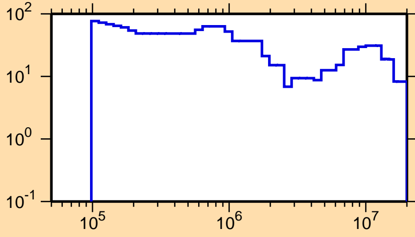
\Delta\sigma/\sigma vs. E for ^{241}\text{U}(n, tot.)
