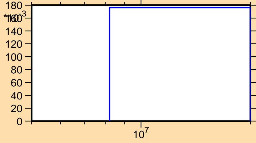
\sigma vs. E for ^{241}\text{U}(n,3n)
