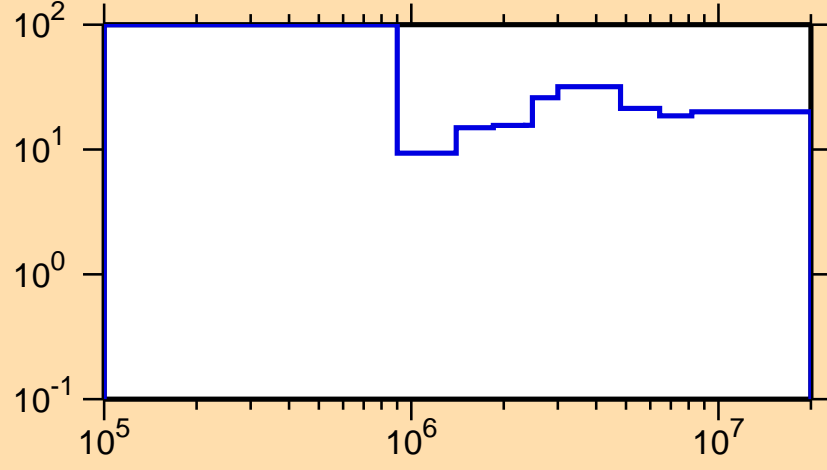
\Delta\sigma/\sigma vs. E for ^{241}\text{U}(n, nonel.)
