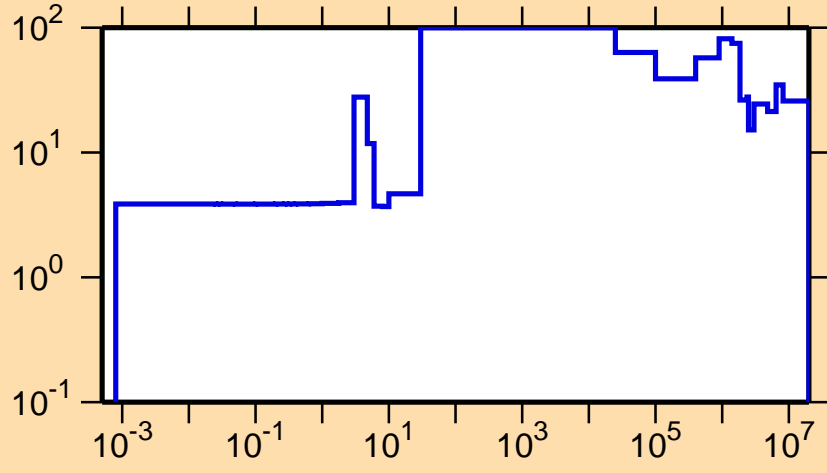
\Delta\sigma/\sigma vs. E for ^{241}\text{U}(n,el.)
