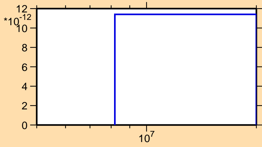
\sigma vs. E for ^{241}\text{U}(n,2np)
