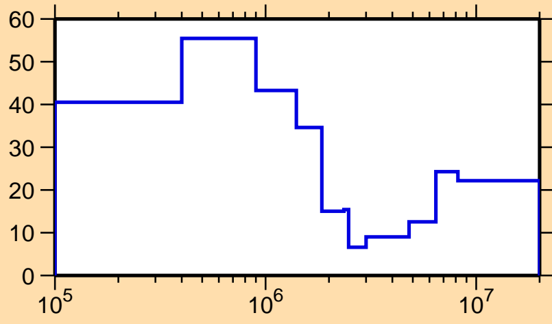
\Delta\sigma/\sigma vs. E for ^{241}\text{U}(n, tot.)
