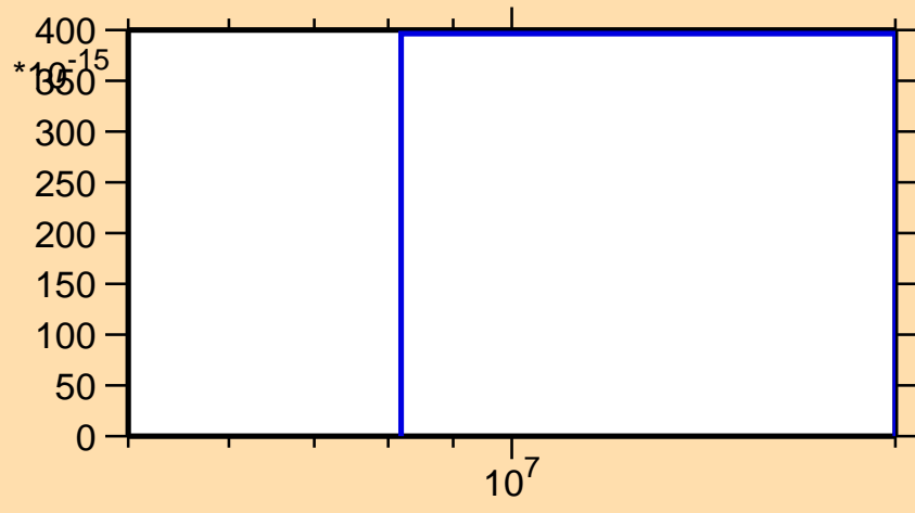
\sigma vs. E for ^{241}\text{U}(n,3n\alpha)
