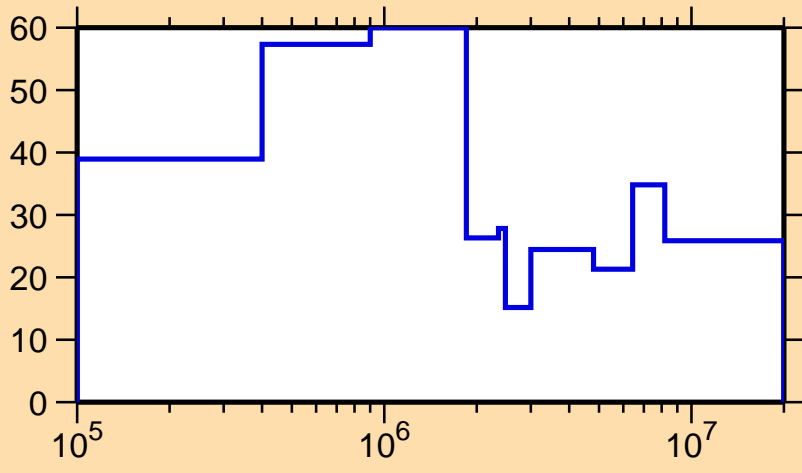
\Delta\sigma/\sigma vs. E for ^{241}\text{U}(n,\text{el.})
