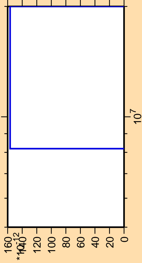
\Delta\sigma/\sigma vs. E for ^{241}\text{U} (mt 42)
