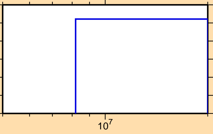
\sigma vs. E for ^{241}\text{U}(n,\text{nd})
