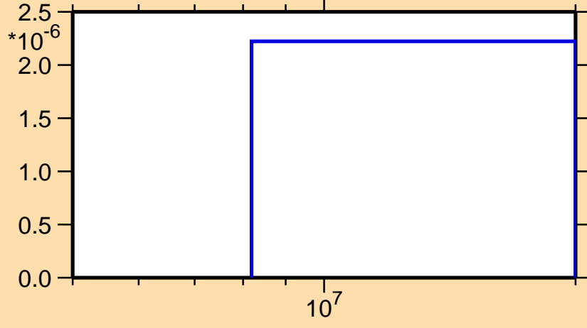
\sigma vs. E for ^{241}\text{U}(n,np)
