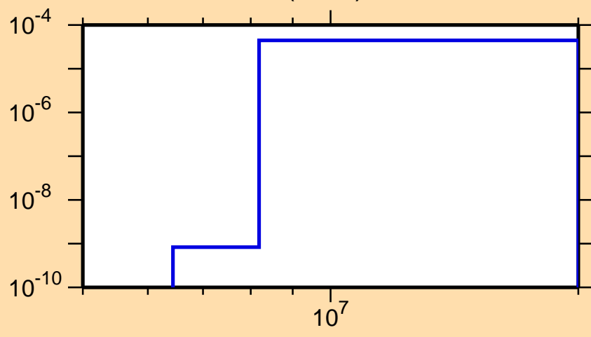
\sigma vs. E for ^{241}\text{U}(n,n\alpha)
