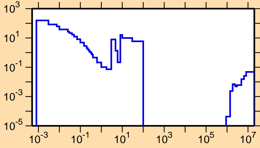
\sigma vs. E for ^{241}\text{U}(n,f)
