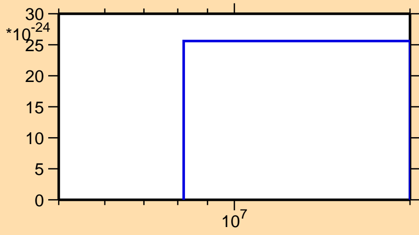
\sigma vs. E for ^{241}\text{U} (mt 42)
