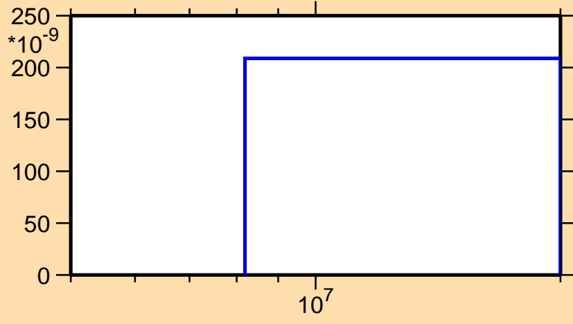
\sigma vs. E for ^{241}\text{U}(n,2n\alpha)
