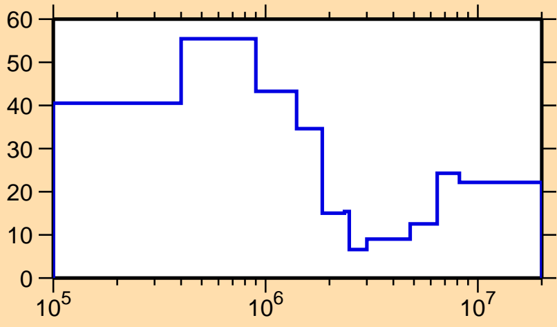
\Delta\sigma/\sigma vs. E for ^{241}\text{U}(n,\text{tot.})
