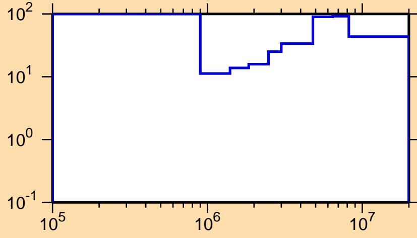
\Delta\sigma/\sigma vs. E for ^{241}\text{U}(n, inel.)
