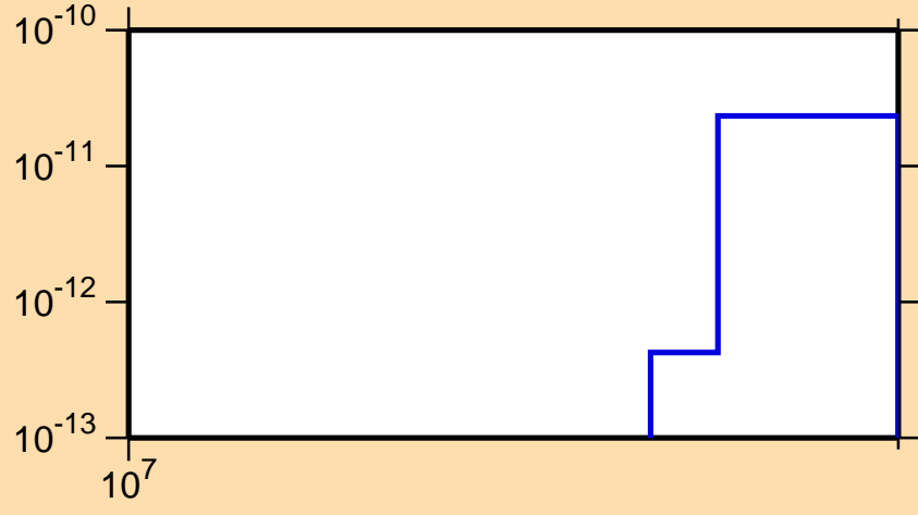
\sigma vs. E for ^{242}\text{U}(n,3n\alpha)
