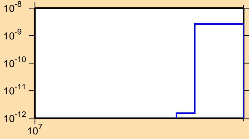
\sigma vs. E for ^{242}\text{U}(n,2np)
