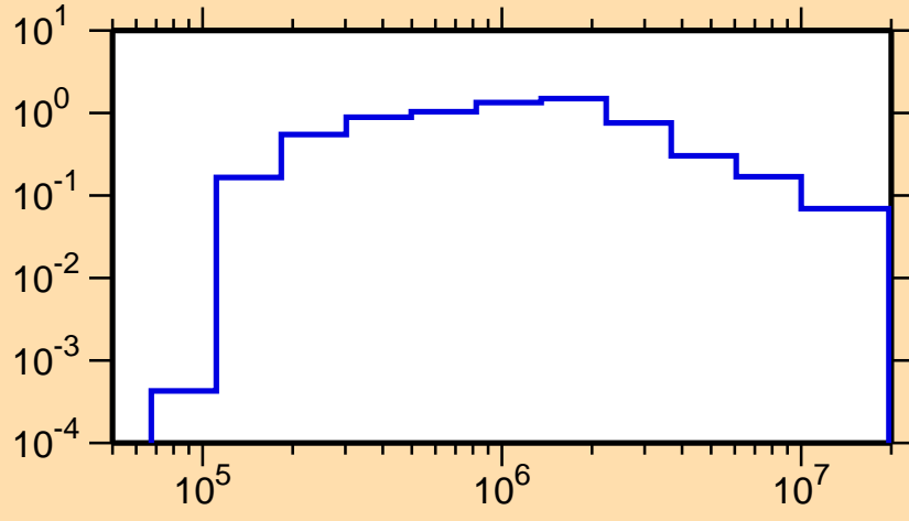
\sigma vs. E for ^{242}\text{U}(n,n_1)
