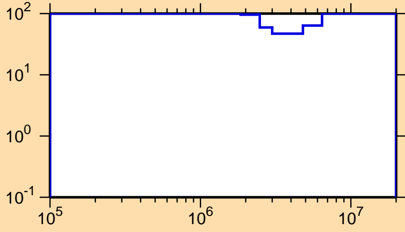
\Delta\sigma/\sigma vs. E for ^{242}\text{U}(n,n\text{cont.})
