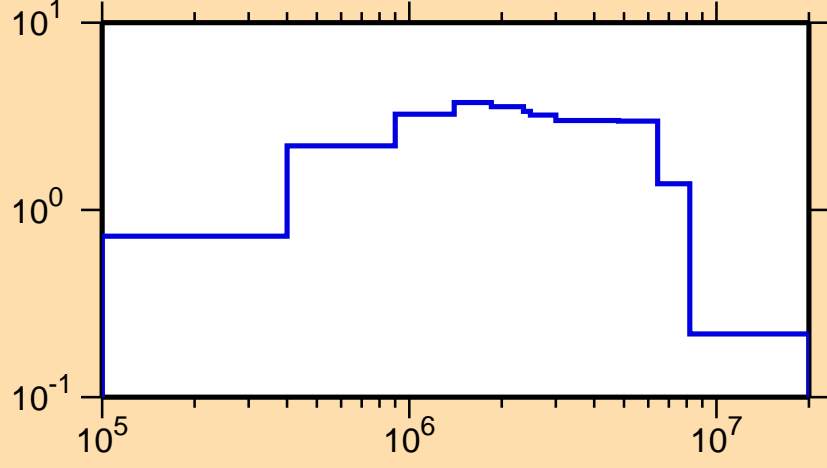
\sigma vs. E for ^{242}\text{U}(n,\text{inel.})
