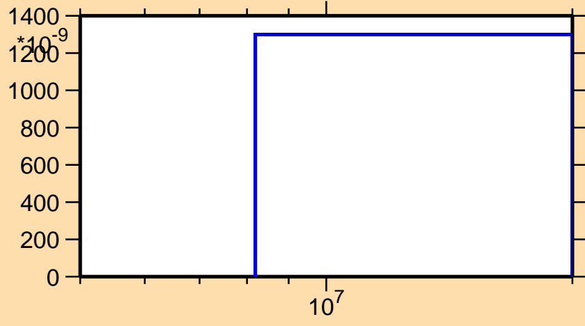
\sigma vs. E for ^{242}\text{U}(n,t)
