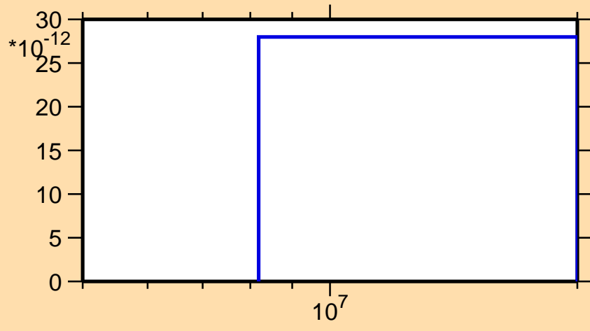
\sigma vs. E for ^{242}\text{U}(n,\text{nd})
