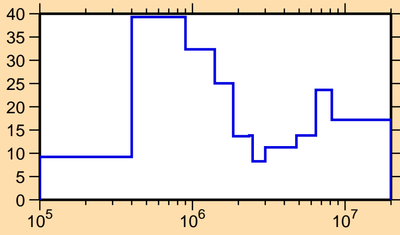
\Delta\sigma/\sigma vs. E for ^{242}\text{U}(n, tot.)
