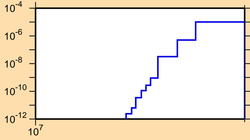
\sigma vs. E for ^{243}\text{U}(n,nd)
