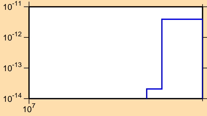
\sigma vs. E for ^{243}\text{U}(n,\text{He3})
