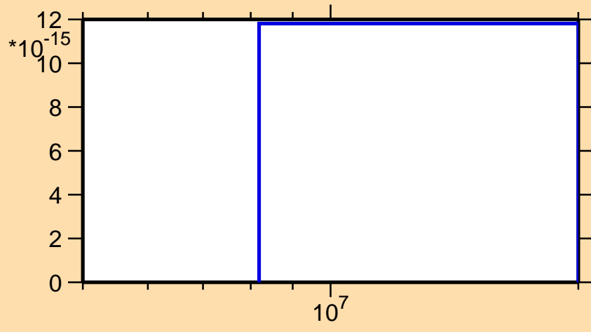
\sigma vs. E for ^{243}\text{U}(n,3n\alpha)
