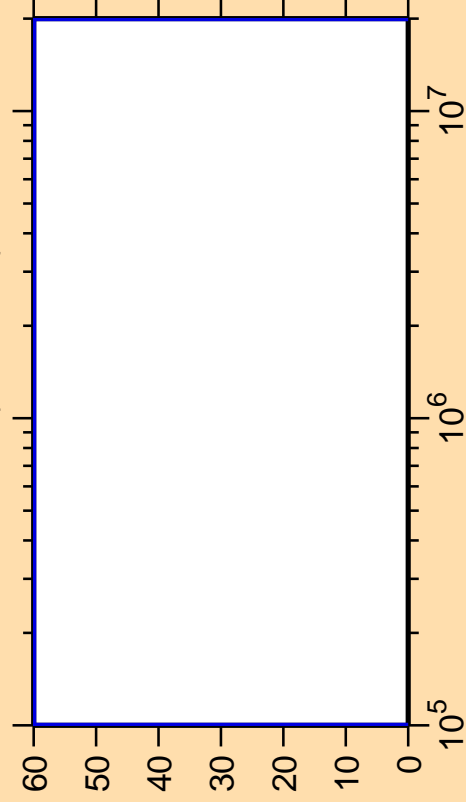
\Delta\sigma/\sigma vs. E for ^{243}\text{U}(n,\text{ncont.})
