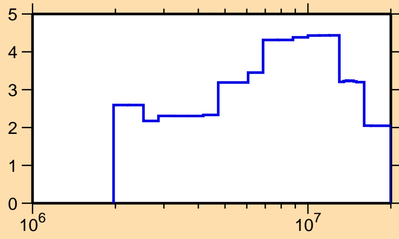
\Delta\sigma/\sigma vs. E for ^{50}\text{V}(n,\text{el.})
