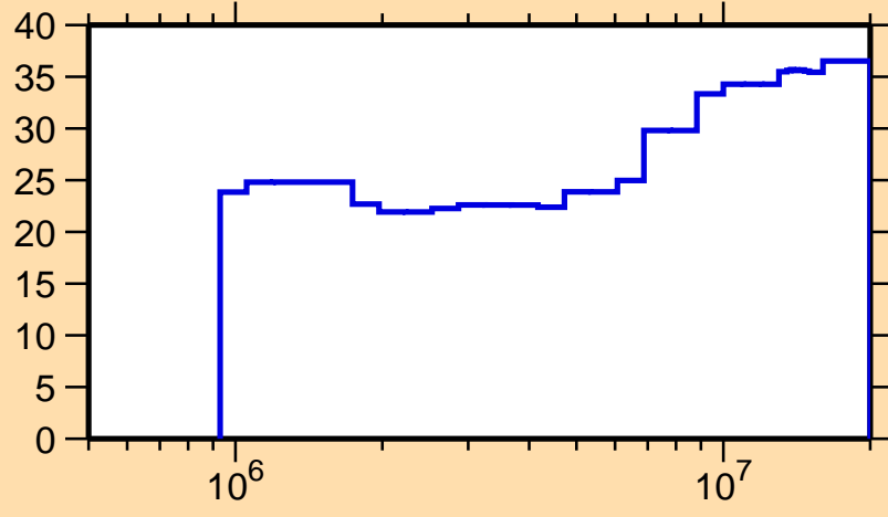
\Delta\sigma/\sigma vs. E for ^{50}\text{V}(n,\gamma)
