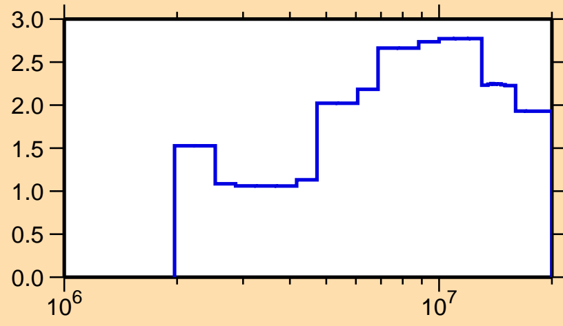
\Delta\sigma/\sigma vs. E for ^{50}\text{V}(n, tot.)
