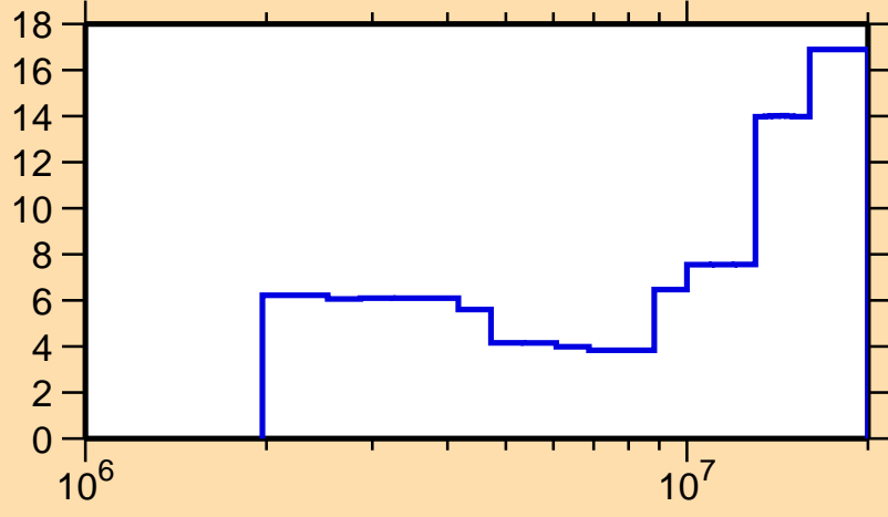
\Delta\sigma/\sigma vs. E for ^{50}\text{V}(n,n\text{cont.})
