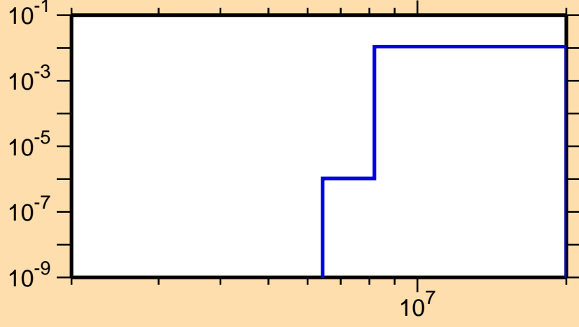
\sigma vs. E for ^{50}\text{V}(n,d)
