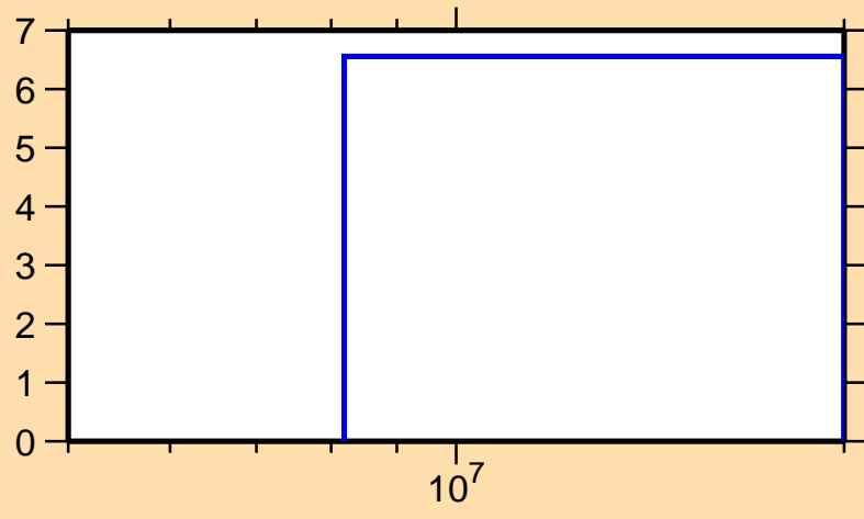
\Delta\sigma/\sigma vs. E for ^{50}\text{V}(n,\text{inel.})
