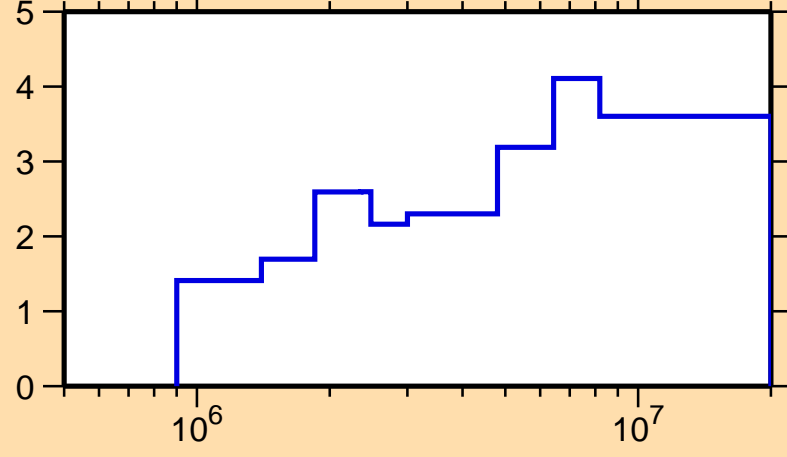
\Delta\sigma/\sigma vs. E for ^{50}\text{V}(n,\text{el.})
