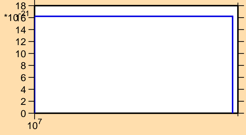
\sigma vs. E for ^{51}\text{V}(n,pd)
