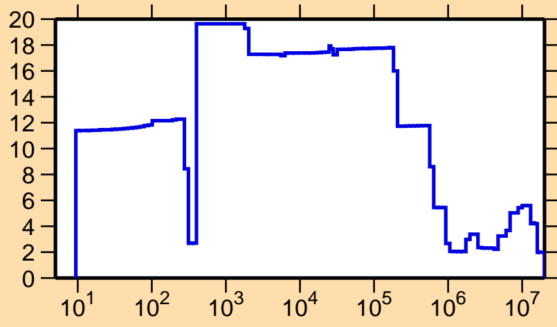
\Delta\sigma/\sigma vs. E for ^{52}\text{V}(n,\text{el.})
