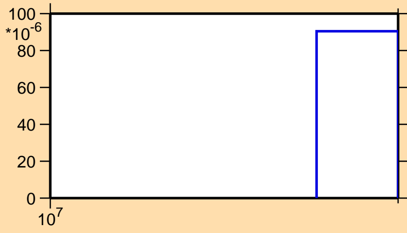
\sigma vs. E for ^{52}\text{V}(n,3n)
