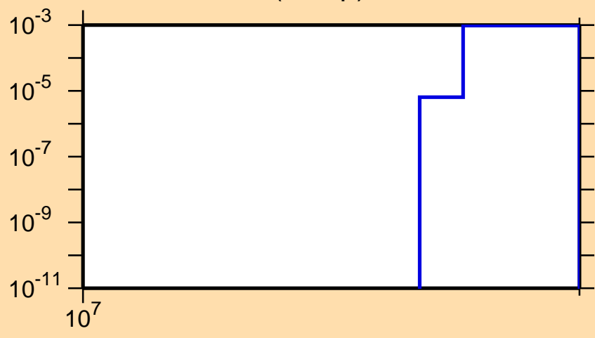
\sigma vs. E for ^{52}\text{V}(n,2np)
