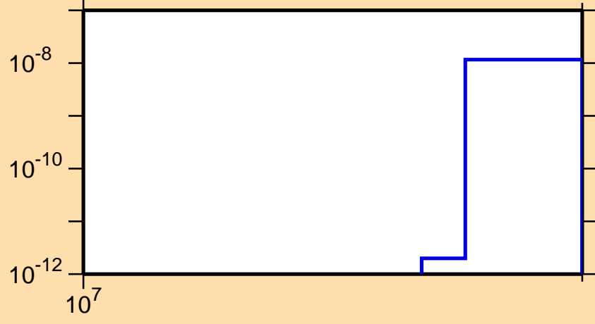
\sigma vs. E for ^{52}\text{V}(n,\text{He}3)
