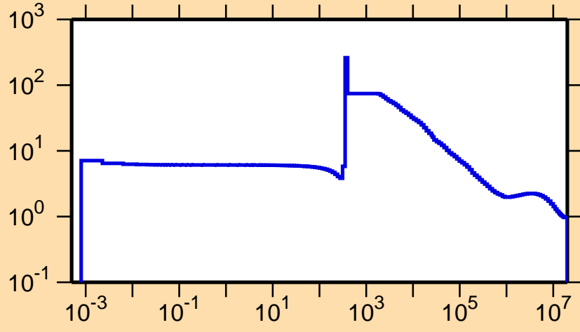
\sigma vs. E for ^{52}\text{V}(n,\text{el.})
