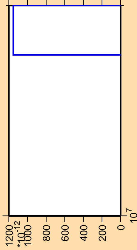
\Delta\sigma/\sigma vs. E for ^{52}\text{V}(n,\text{pt})
