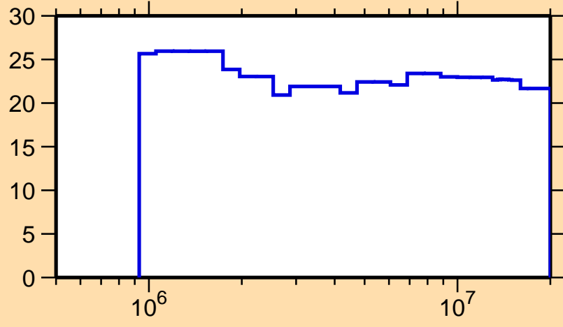
\Delta\sigma/\sigma vs. E for ^{52}\text{V}(n,\gamma)
