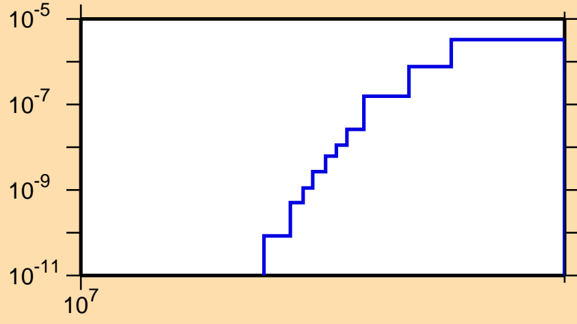
\sigma vs. E for ^{52}\text{V}(n,p\alpha)
