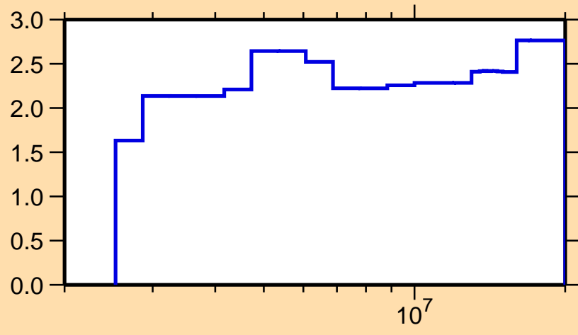
\Delta\sigma/\sigma vs. E for ^{52}\text{V}(n,n\text{onel.})
