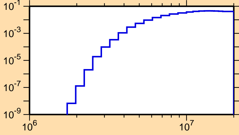
\sigma vs. E for ^{52}\text{V}(n,p)
