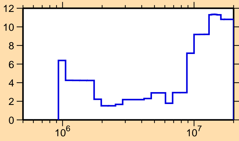
\Delta\sigma/\sigma vs. E for ^{52}\text{V}(n,\text{inel.})
