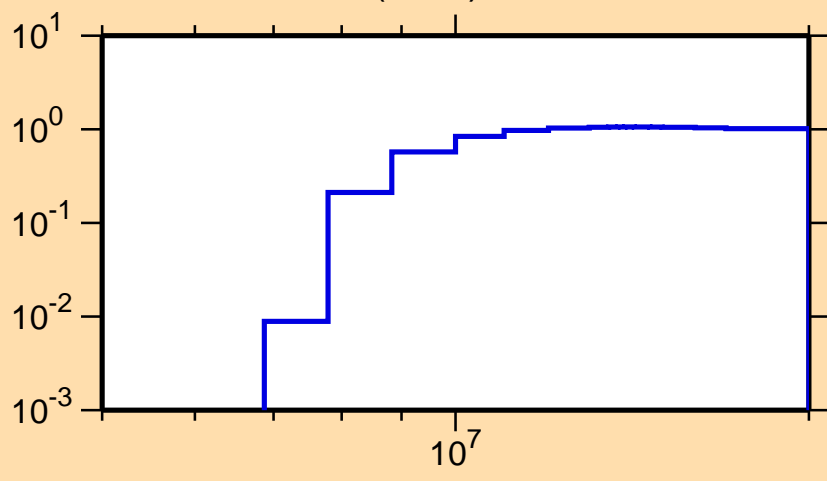
\sigma vs. E for ^{52}\text{V}(n,2n)
