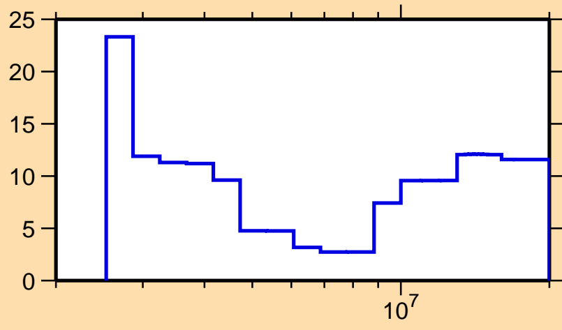
\Delta\sigma/\sigma vs. E for ^{52}\text{V}(n,n\text{cont.})
