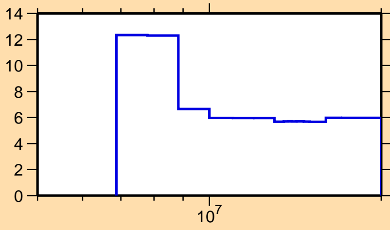
\Delta\sigma/\sigma vs. E for ^{52}\text{V}(n,2n)
