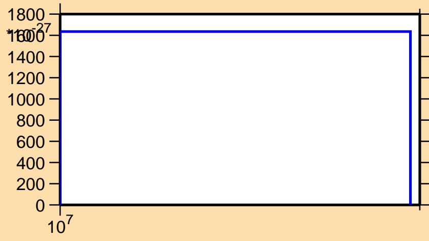
\sigma vs. E for ^{52}\text{V}(n,pt)
