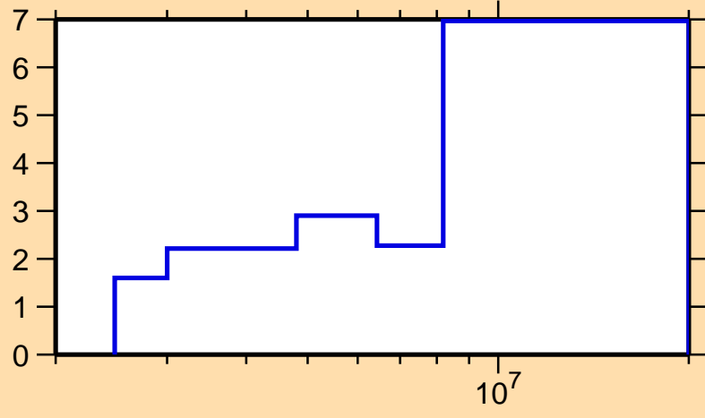
\Delta\sigma/\sigma vs. E for ^{52}\text{V}(n,\text{inel.})
