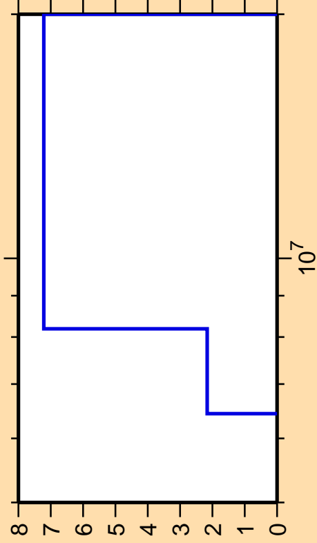
\Delta\sigma/\sigma vs. E for ^{52}\text{V}(n,n\text{cont.})
