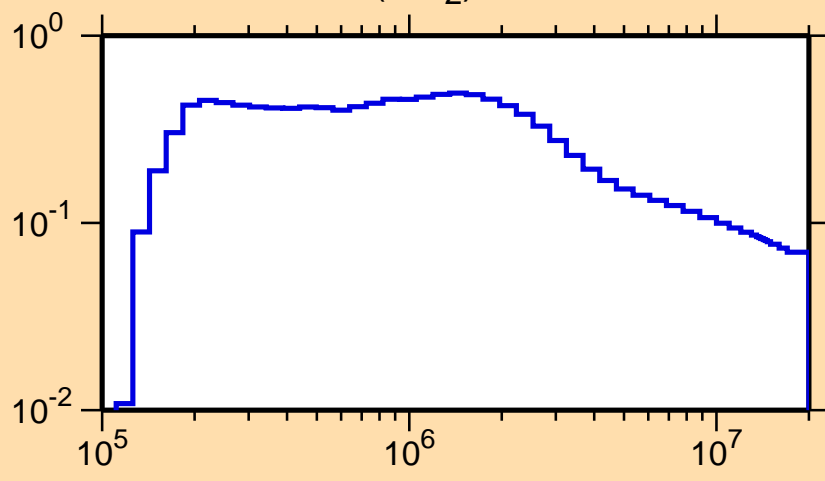
\sigma vs. E for ^{54}\text{V}(n,n_2)
