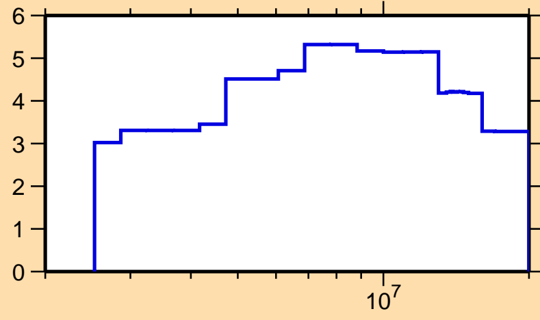
\Delta\sigma/\sigma vs. E for ^{54}\text{V}(n,el.)
