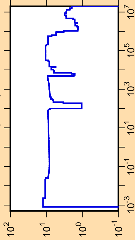
\Delta\sigma/\sigma vs. E for ^{54}\text{V}(n,\text{tot.})
