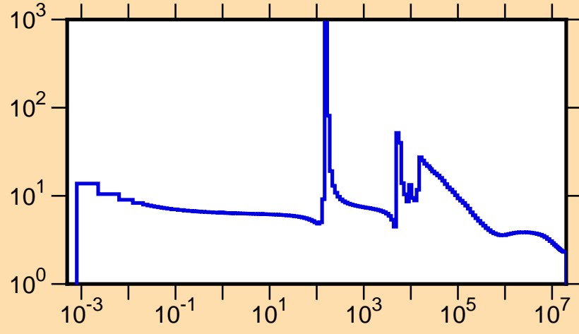
\sigma vs. E for ^{54}\text{V}(n,\text{tot.})
