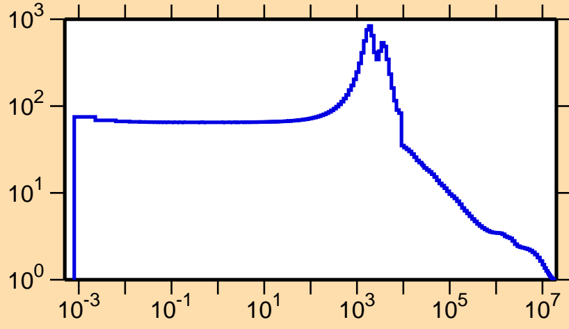
\sigma vs. E for ^{55}\text{V}(n,\text{el.})
