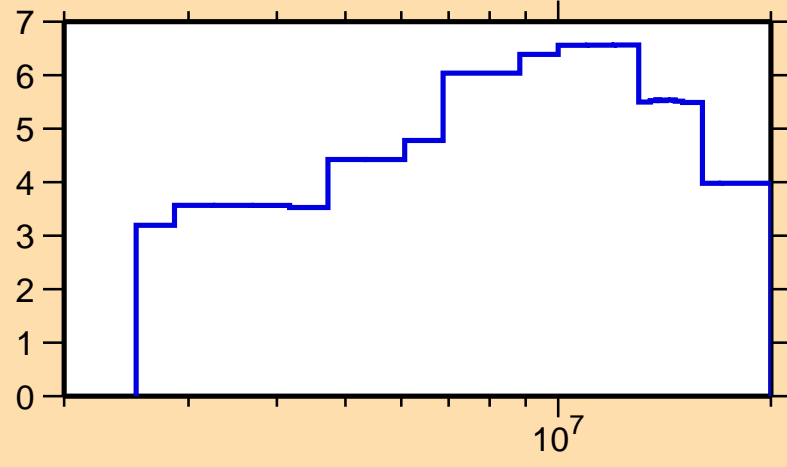
\Delta\sigma/\sigma vs. E for ^{55}\text{V}(n,el.)
