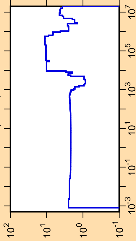
\Delta\sigma/\sigma vs. E for ^{55}\text{V}(n,\text{tot.})
