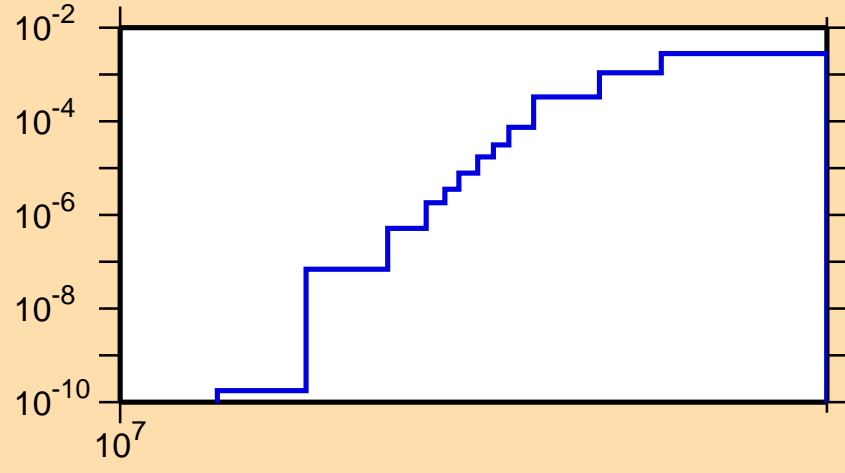
\sigma vs. E for ^{55}\text{V}(n,np)
