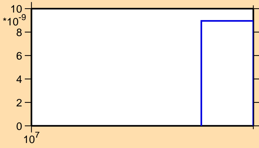
\sigma vs. E for ^{55}\text{V}(n,2np)
