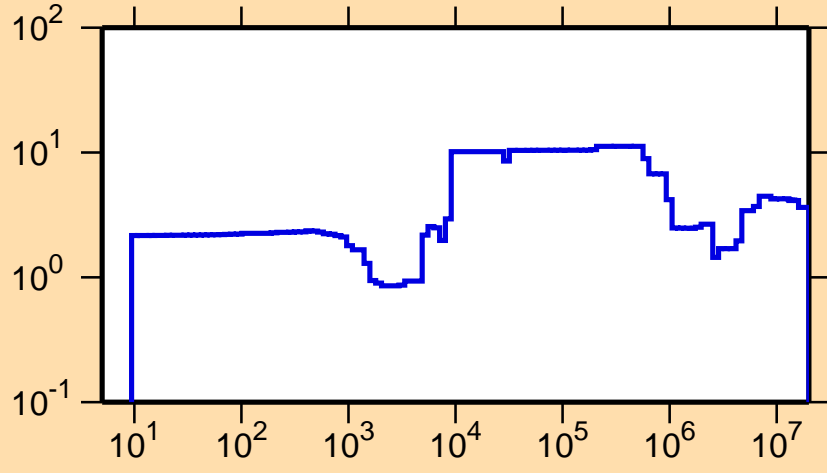
\Delta\sigma/\sigma vs. E for ^{55}\text{V}(n,\text{tot.})
