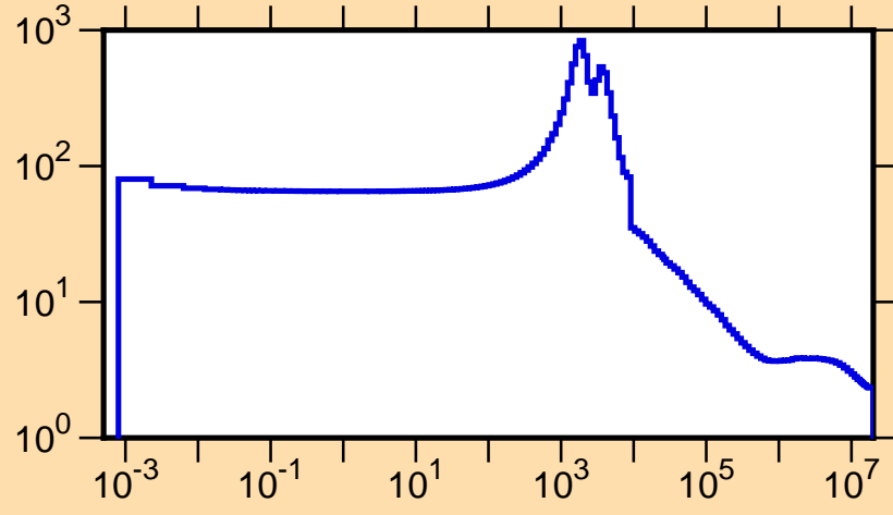
\sigma vs. E for ^{55}\text{V}(n,\text{tot.})
