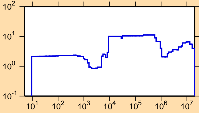
\Delta\sigma/\sigma vs. E for ^{55}\text{V}(n,\text{el.})
