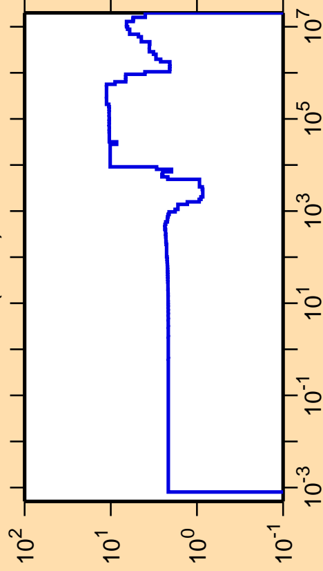
\Delta\sigma/\sigma vs. E for ^{55}\text{V}(n,\text{el.})
