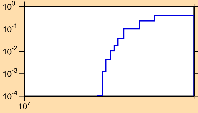
\sigma vs. E for ^{55}\text{V}(n,3n)
