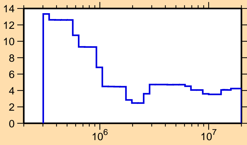
\Delta\sigma/\sigma vs. E for ^{55}\text{V}(n,\text{nonel.})
