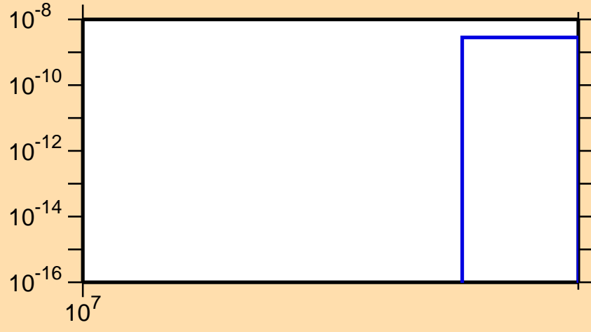
\sigma vs. E for ^{55}\text{V}(n,2n\alpha)
