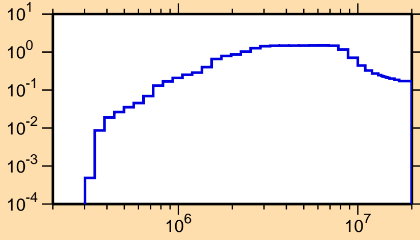
\sigma vs. E for ^{55}\text{V}(n,\text{inel.})
