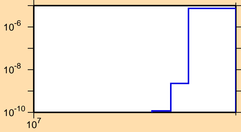
\sigma vs. E for ^{55}\text{V}(n,nd)
