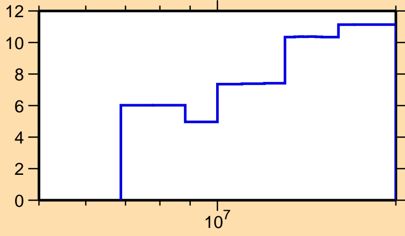
\Delta\sigma/\sigma vs. E for ^{55}\text{V}(n,\text{inel.})
