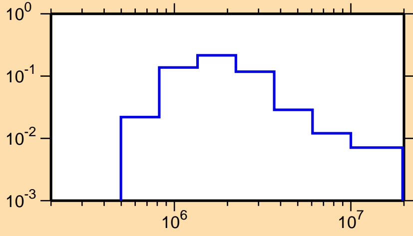
\sigma vs. E for ^{55}\text{V}(n,n_2)
