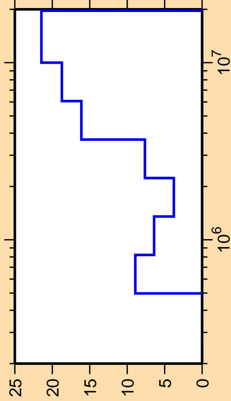
\Delta\sigma/\sigma vs. E for ^{55}\text{V}(n,n_2)
