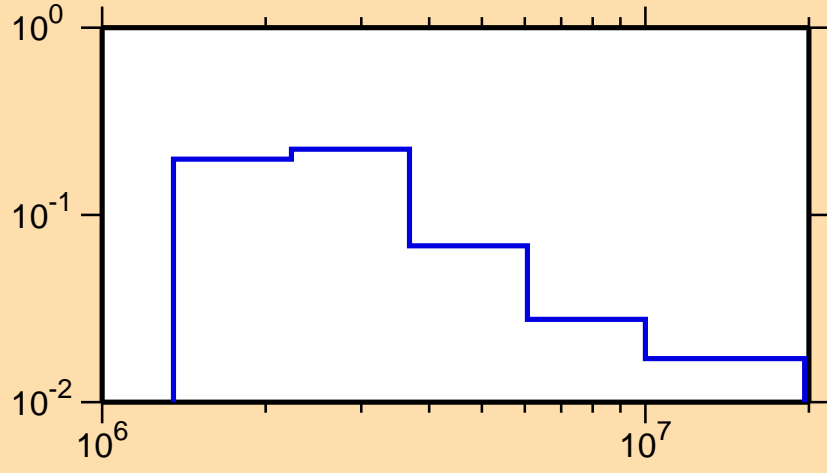
\sigma vs. E for ^{55}\text{V}(n,n_4)
