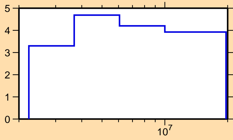
\Delta\sigma/\sigma vs. E for ^{55}\text{V}(n,n\text{onel.})
