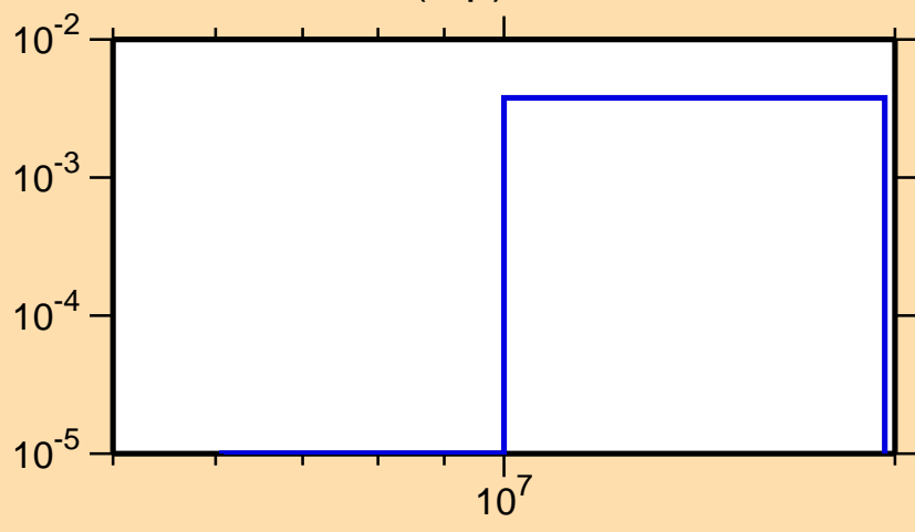
\sigma vs. E for ^{55}\text{V}(n,p)
