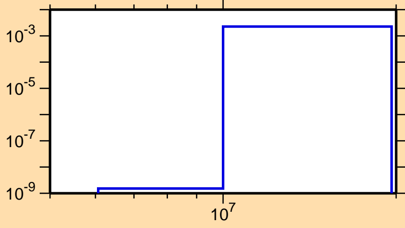
\sigma vs. E for ^{55}\text{V}(n,d)
