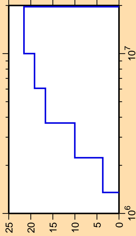
\Delta\sigma/\sigma vs. E for ^{55}\text{V}(n,n_4)
