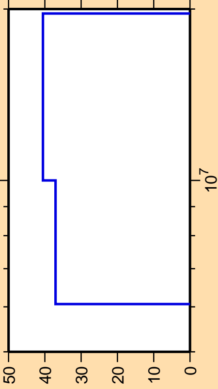
\Delta\sigma/\sigma vs. E for ^{55}\text{V}(n,p)
