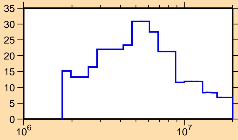
\Delta\sigma/\sigma vs. E for ^{162}\text{W}(n, el.)
