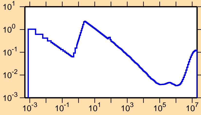
\sigma vs. E for ^{162}\text{W}(n,\alpha)
