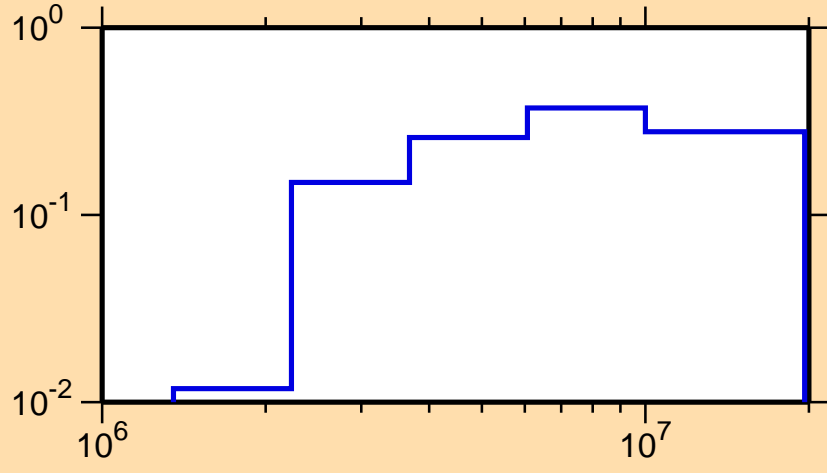
\sigma vs. E for ^{162}\text{W}(n,n\text{cont.})
