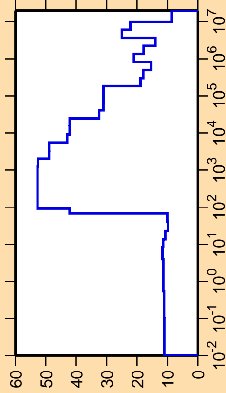
\Delta\sigma/\sigma vs. E for ^{162}\text{W}(n,\text{el.})
