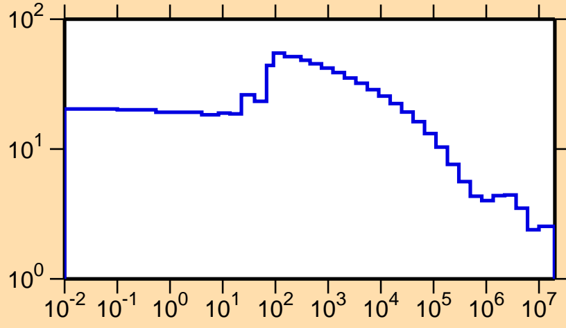
\sigma vs. E for ^{162}\text{W}(n,\text{el.})
