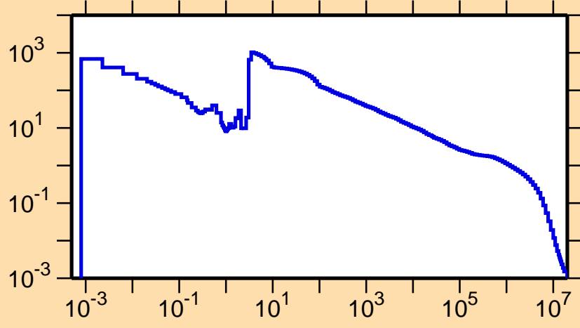
\sigma vs. E for ^{163}\text{W}(n,\gamma)
