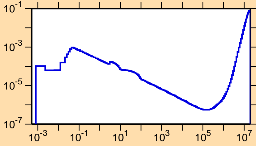
\sigma vs. E for ^{163}\text{W}(n,p\alpha)
