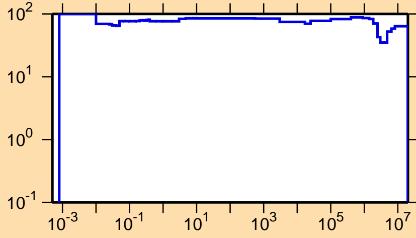
\Delta\sigma/\sigma vs. E for ^{163}\text{W}(n,p)
