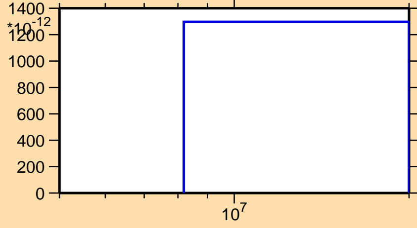
\sigma vs. E for ^{163}\text{W} (mt 34)
