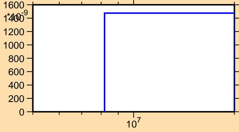
\sigma vs. E for ^{163}\text{W}(n,\text{pt})
