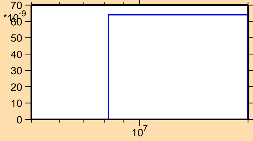
\sigma vs. E for ^{163}\text{W}(\text{mt117})
