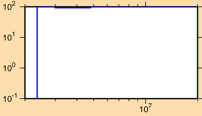
\Delta\sigma/\sigma vs. E for ^{163}\text{W}(n,ncont.)
