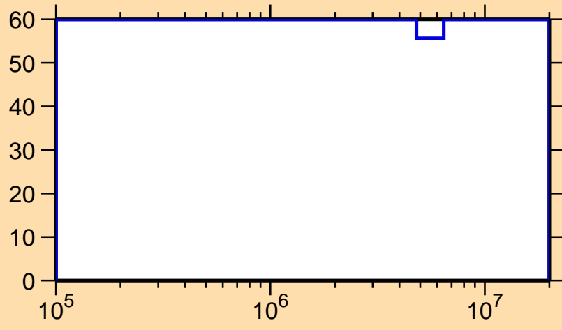
\Delta\sigma/\sigma vs. E for ^{163}\text{W}(n,n_1)
