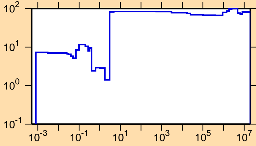
\Delta\sigma/\sigma vs. E for ^{163}\text{W}(n,\gamma)
