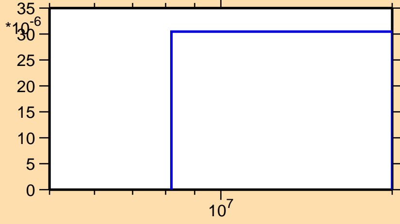
\sigma vs. E for ^{163}\text{W}(n,2n\alpha)
