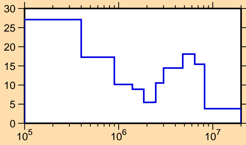
\Delta\sigma/\sigma vs. E for ^{163}\text{W}(n,\text{tot.})
