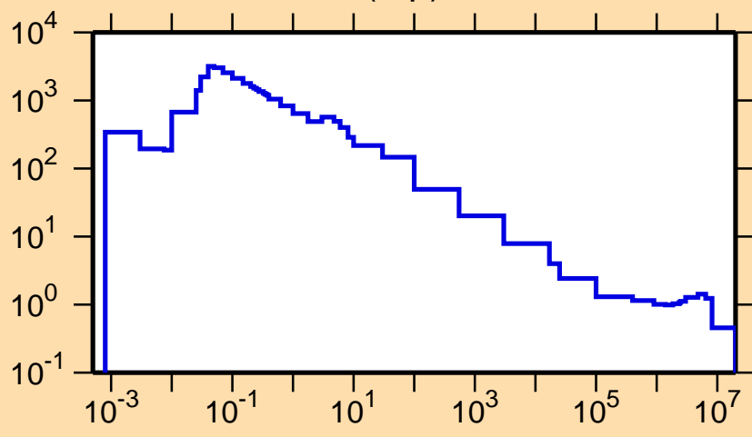
\sigma vs. E for ^{163}\text{W}(n,p)
