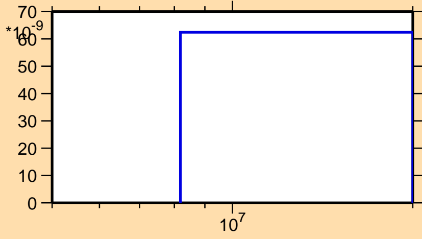
\sigma vs. E for ^{163}\text{W}(n,\text{nd})
