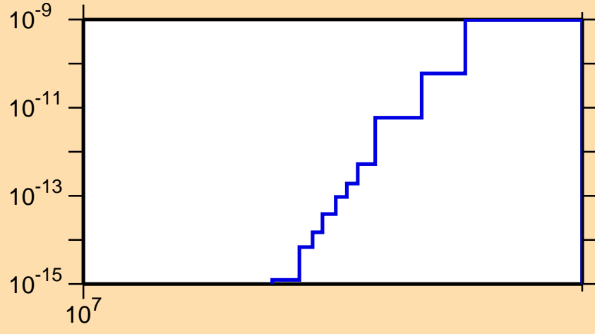
\sigma vs. E for ^{164}\text{W} (mt 34)
