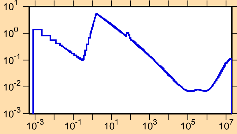
\sigma vs. E for ^{164}\text{W}(n,\alpha)
