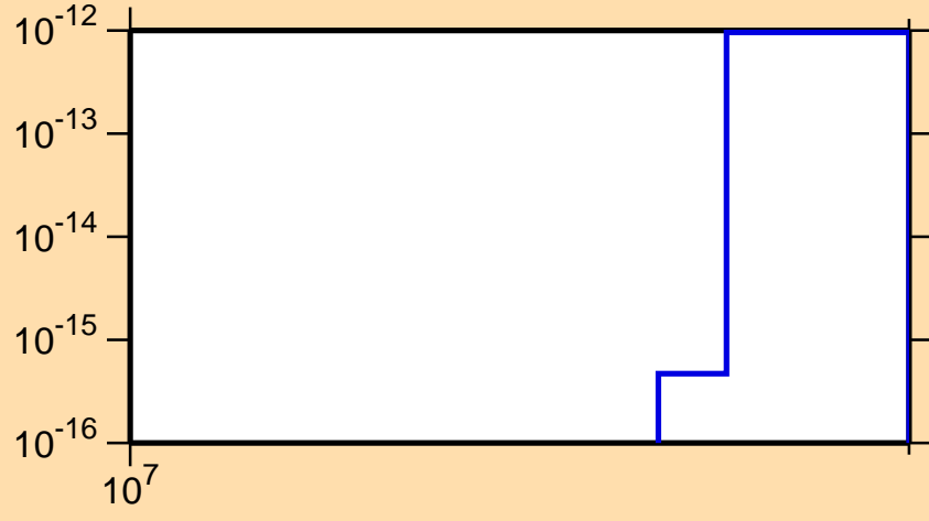
\sigma vs. E for ^{164}\text{W}(n,nt)
