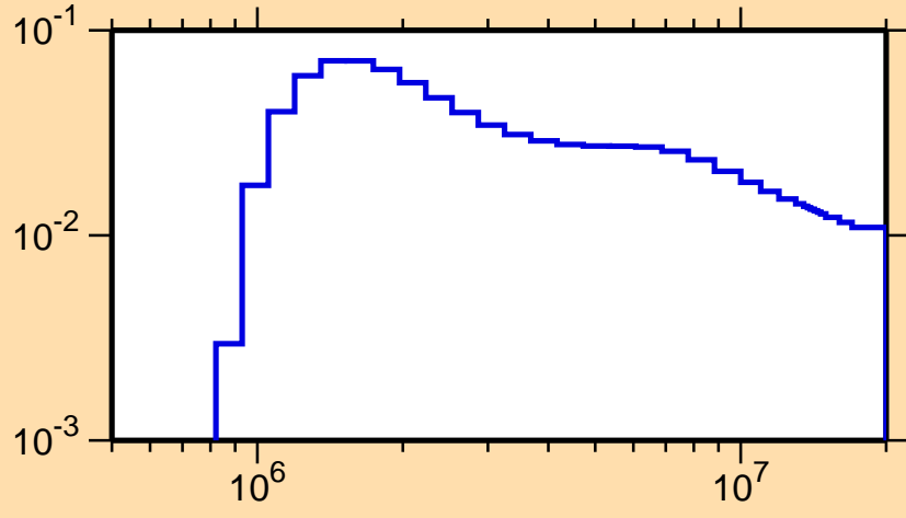
\sigma vs. E for ^{164}\text{W}(n,n_2)
