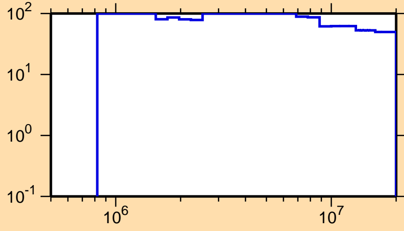
\Delta\sigma/\sigma vs. E for ^{164}\text{W}(n,ncont.)
