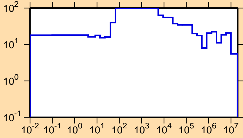
\Delta\sigma/\sigma vs. E for ^{164}\text{W}(n,el.)
