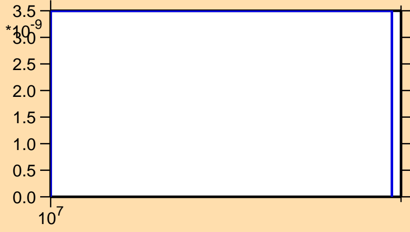
\sigma vs. E for ^{164}\text{W}(n,\text{pt})
