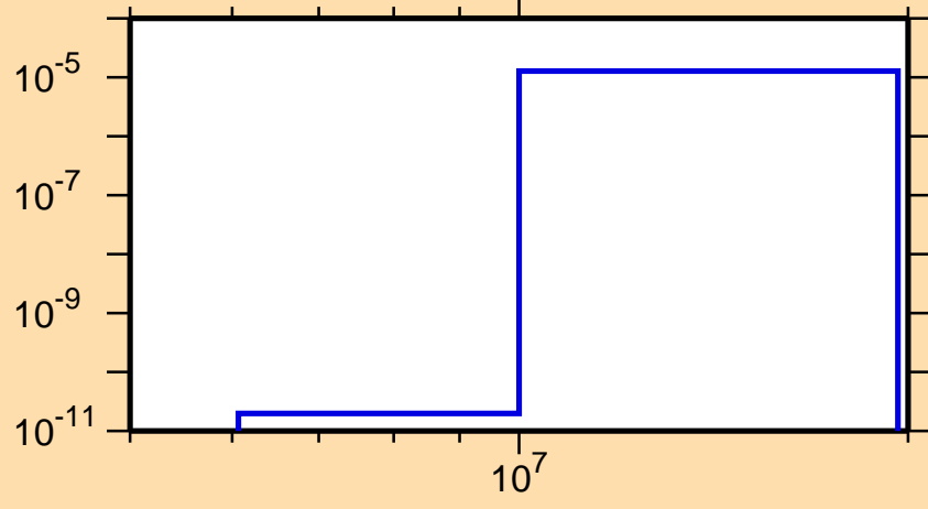
\sigma vs. E for ^{164}\text{W} (mt 45)
