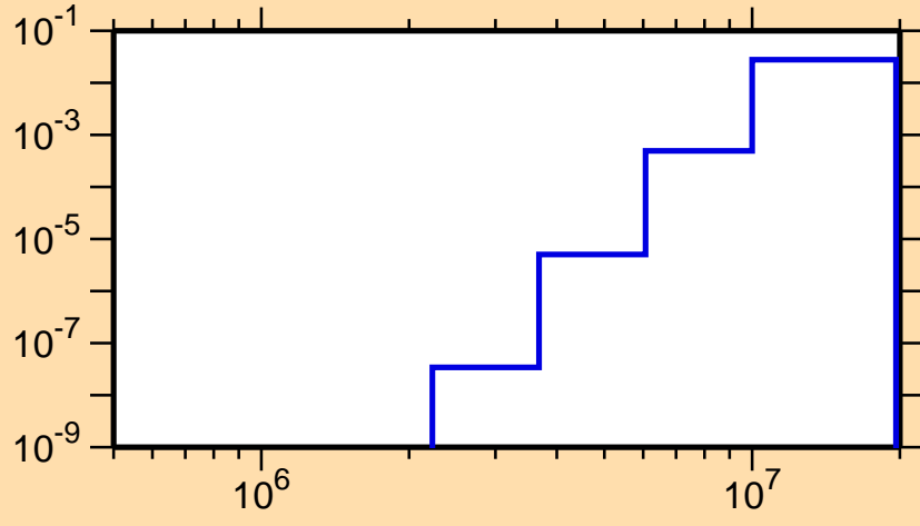
\sigma vs. E for ^{164}\text{W}(n,n\alpha)
