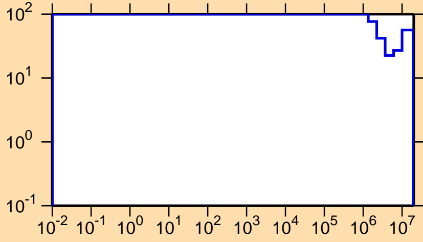
\Delta\sigma/\sigma vs. E for ^{164}\text{W}(n,p)
