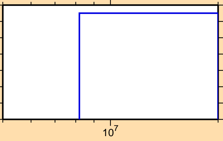
\sigma vs. E for ^{164}\text{W}(n,2n\alpha)
