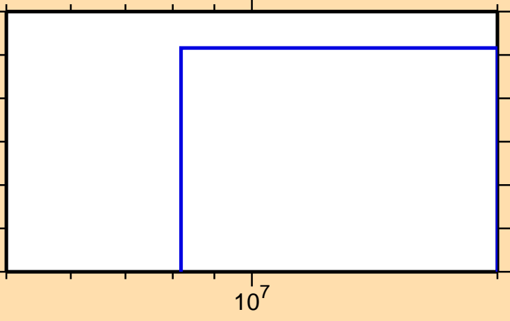
\sigma vs. E for ^{164}\text{W}(n,t)
