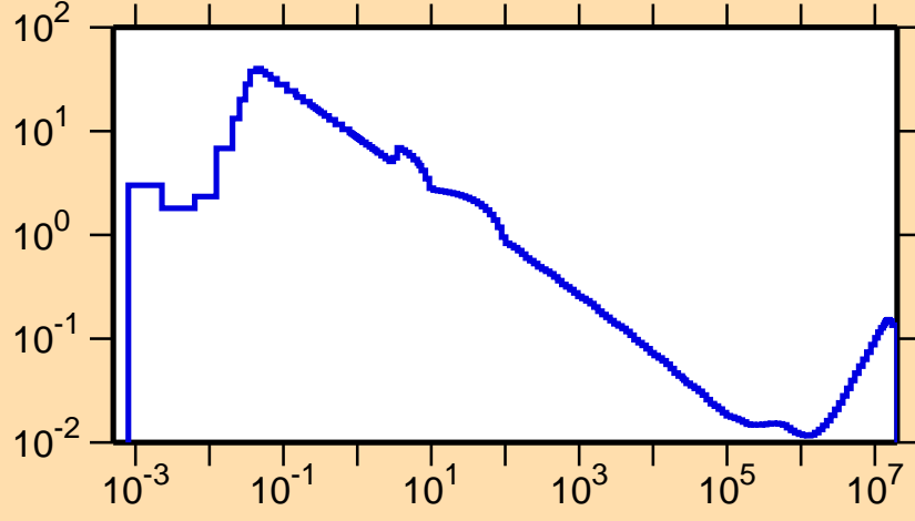
\sigma vs. E for ^{165}\text{W}(n,\alpha)
