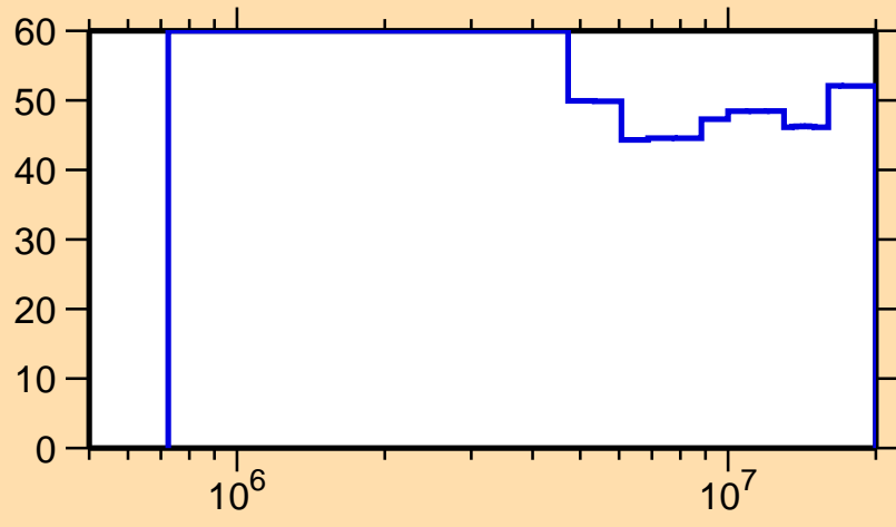
\Delta\sigma/\sigma vs. E for ^{165}\text{W}(n,ncont.)
