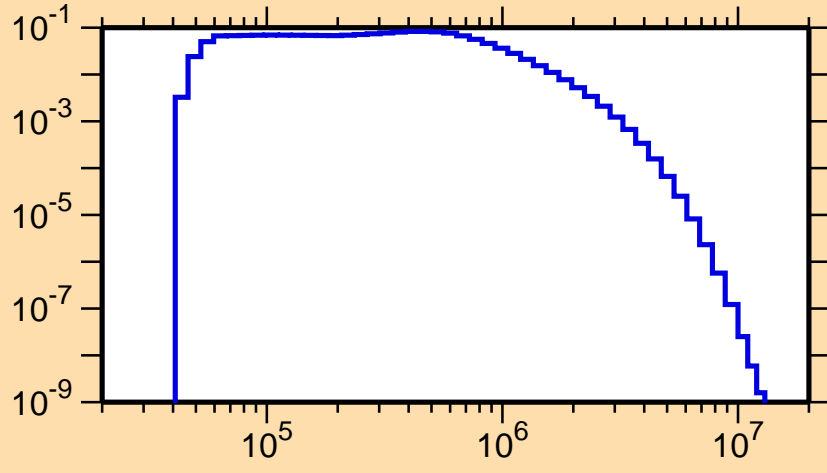
\sigma vs. E for ^{165}\text{W}(n,n_1)
