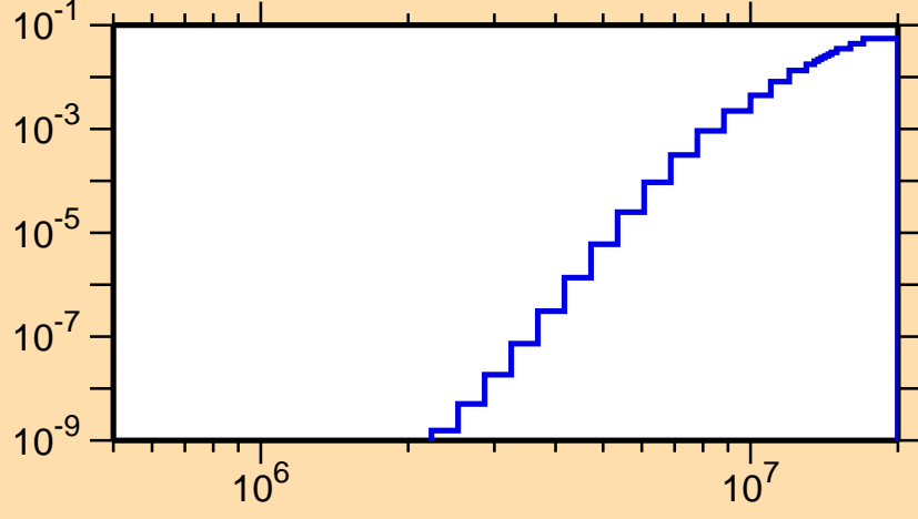
\sigma vs. E for ^{165}\text{W}(n,n\alpha)
