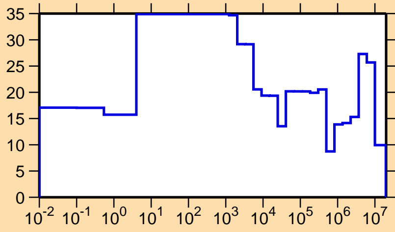
\Delta\sigma/\sigma vs. E for ^{165}\text{W}(n,el.)
