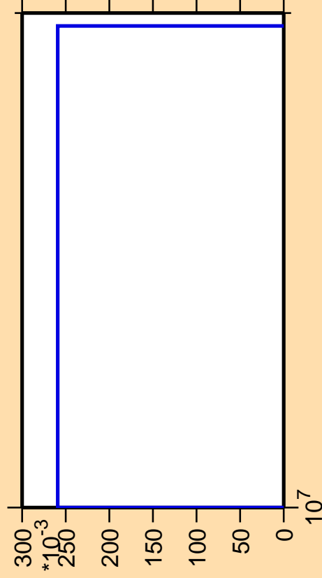
\Delta\sigma/\sigma vs. E for ^{165}\text{W}(n,nt)
