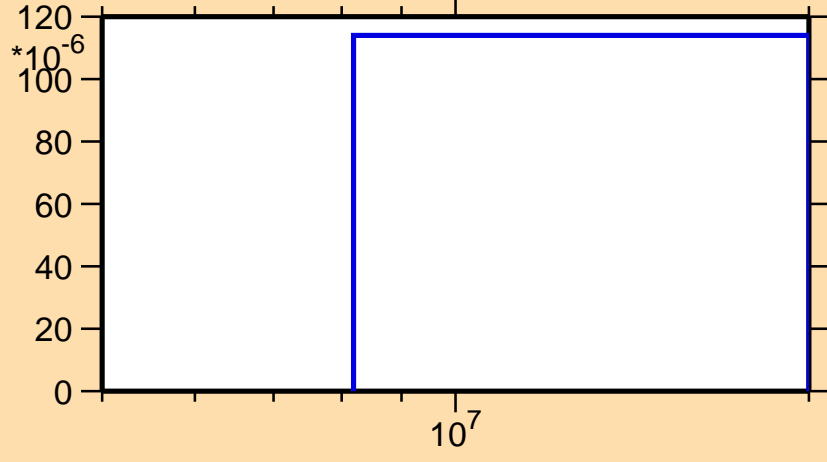
\sigma vs. E for ^{165}\text{W}(n,2np)
