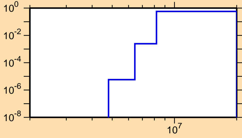
\sigma vs. E for ^{165}\text{W}(n,np)
