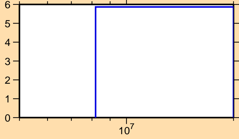
\Delta\sigma/\sigma vs. E for ^{165}\text{W}(n,\text{nonel.})
