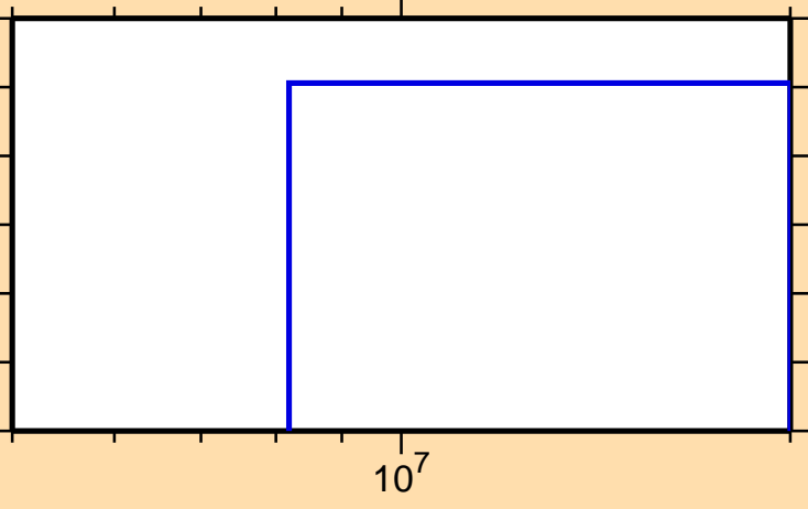
\sigma vs. E for ^{165}\text{W}(n,\text{nd})
