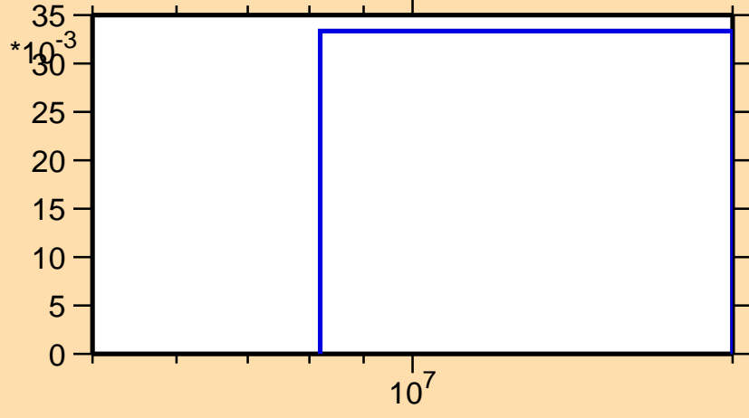
\sigma vs. E for ^{165}\text{W}(n,2n)
