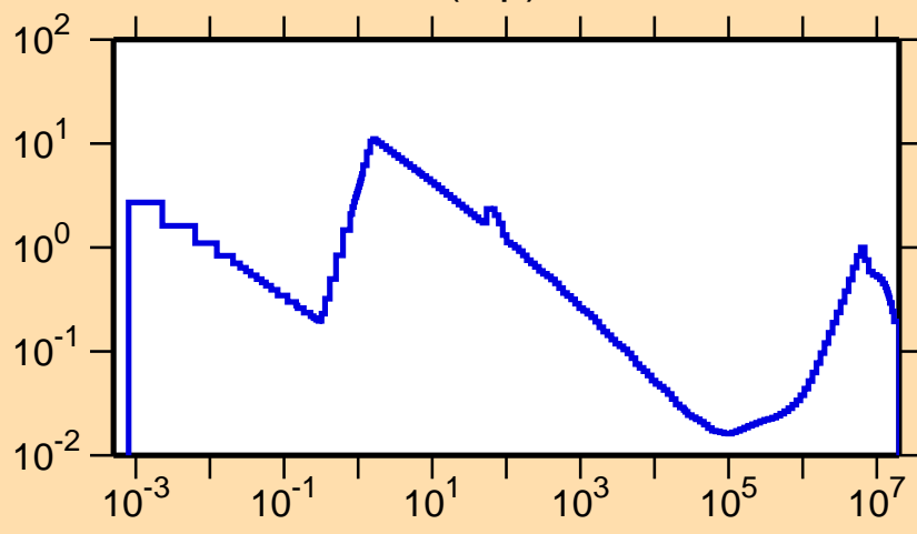
\sigma vs. E for ^{166}\text{W}(n,p)
