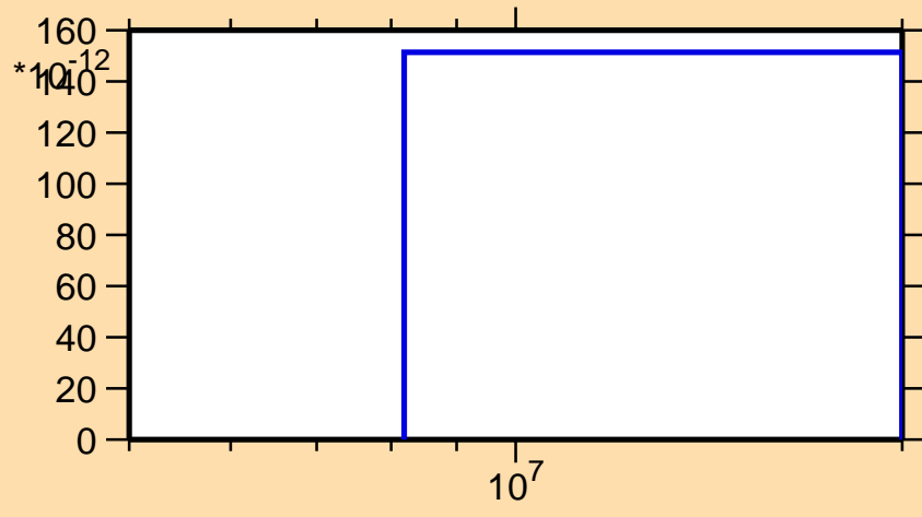
\sigma vs. E for ^{166}\text{W}(n,\text{pt})
