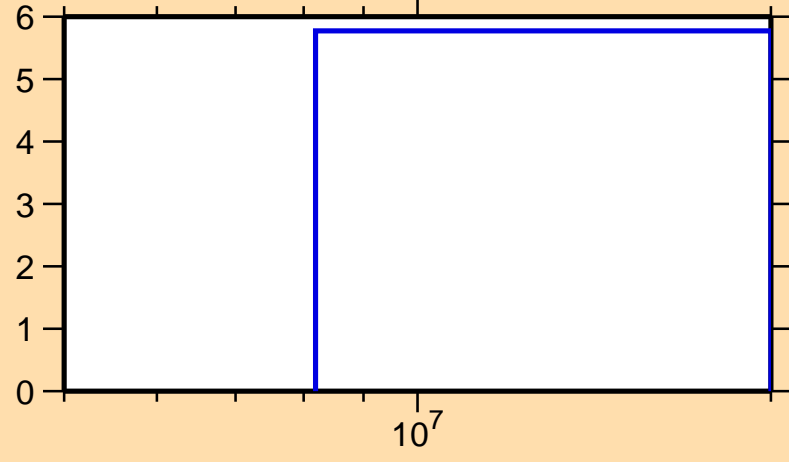
\Delta\sigma/\sigma vs. E for ^{166}\text{W}(n,\text{nonel.})
