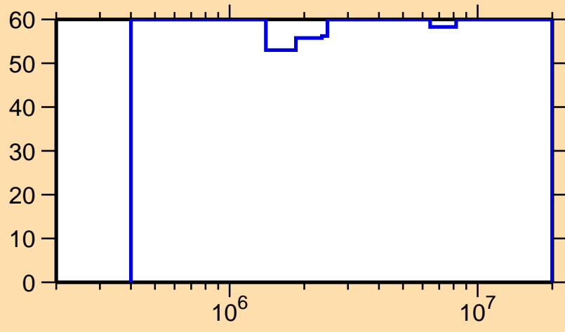
\Delta\sigma/\sigma vs. E for ^{166}\text{W}(n,n\text{cont.})
