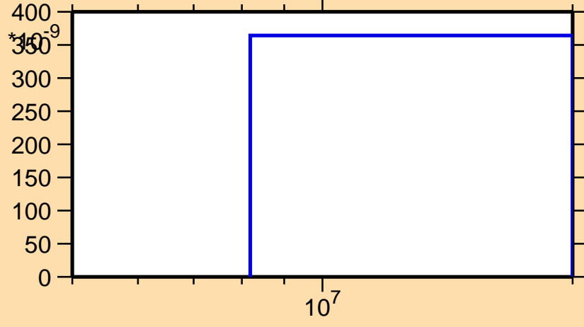
\sigma vs. E for ^{166}\text{W}(n,2np)
