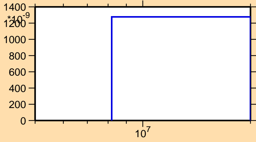
\sigma vs. E for ^{166}\text{W}(n,\text{pd})
