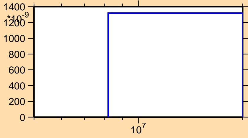
\sigma vs. E for ^{166}\text{W} (mt 45)
