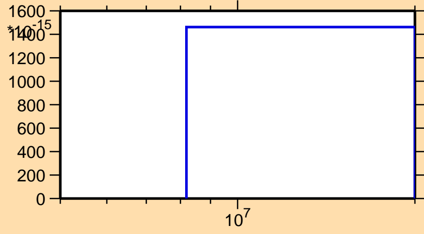
\sigma vs. E for ^{166}\text{W} (mt 34)
