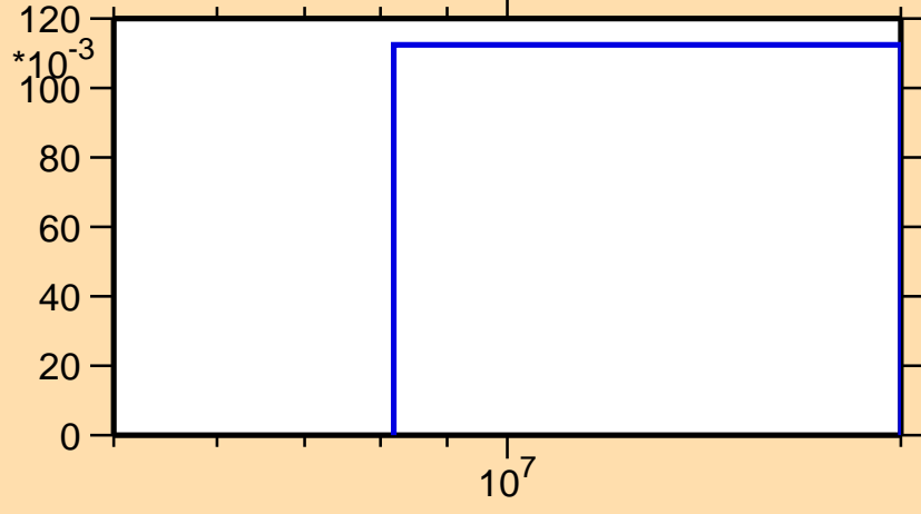
\sigma vs. E for ^{166}\text{W}(n,2n)
