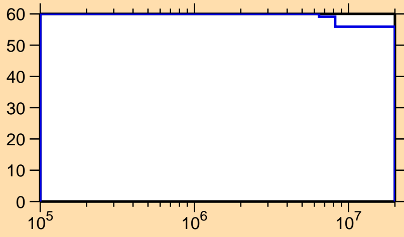
\Delta\sigma/\sigma vs. E for ^{166}\text{W}(n,n_1)
