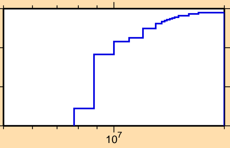
\sigma vs. E for ^{167}\text{W}(n,2n)
