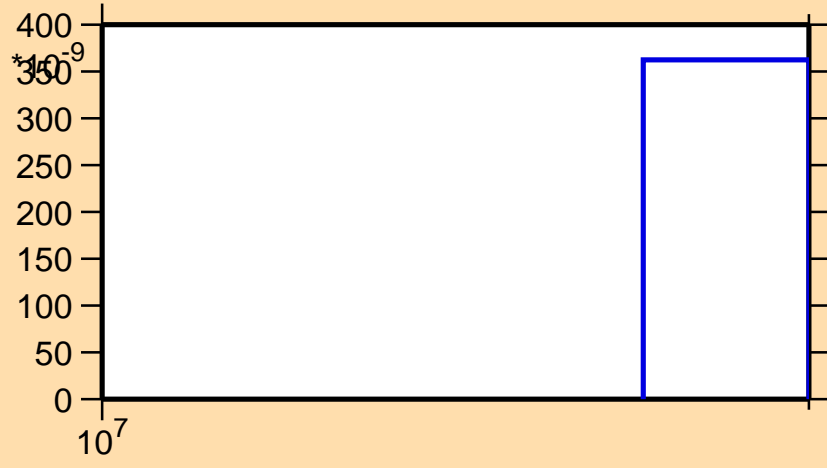
\sigma vs. E for ^{167}\text{W}(n,3n)
