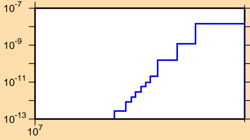
\sigma vs. E for ^{167}\text{W} (mt 34)
