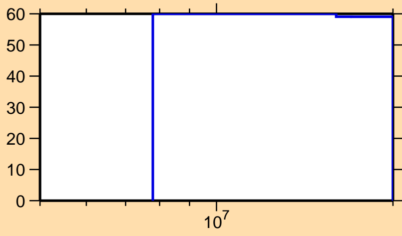
\Delta\sigma/\sigma vs. E for ^{167}\text{W}(n,2n)
