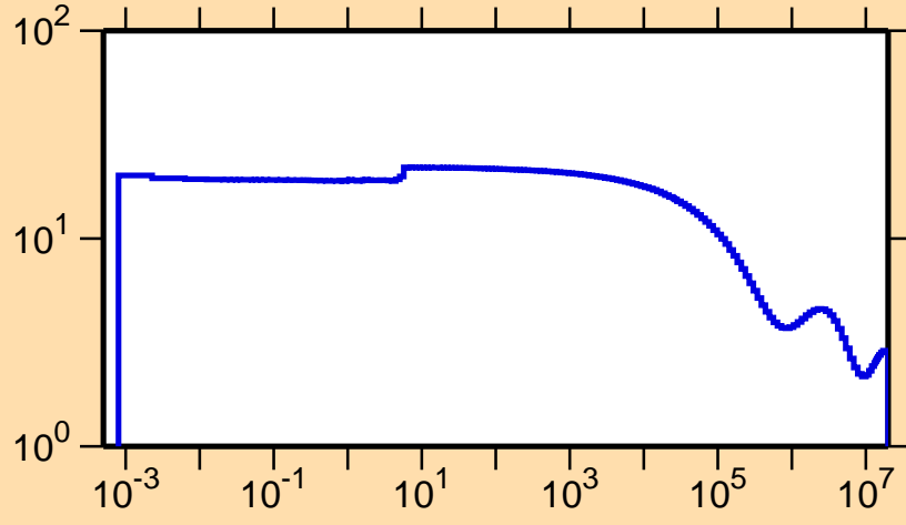
\sigma vs. E for ^{167}\text{W}(n,\text{el.})
