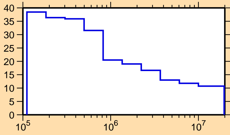
\Delta\sigma/\sigma vs. E for ^{167}\text{W}(n, nonel.)
