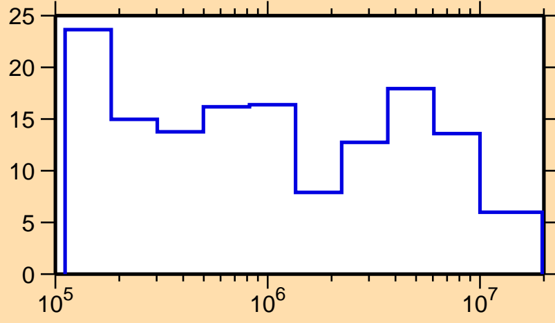
\Delta\sigma/\sigma vs. E for ^{167}\text{W}(n, tot.)
