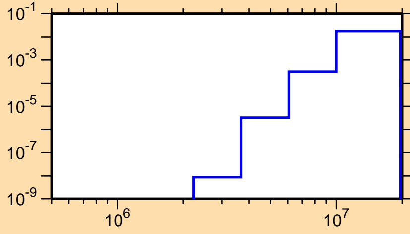
\sigma vs. E for ^{167}\text{W}(n,n\alpha)
