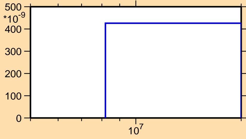
\sigma vs. E for ^{167}\text{W} (mt 45)
