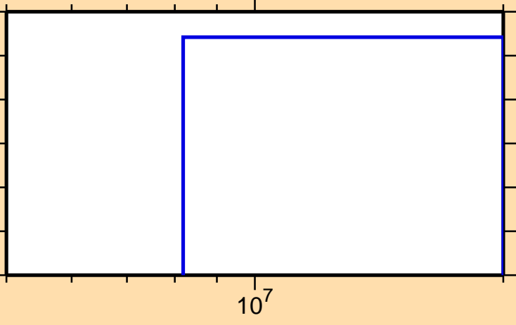
\sigma vs. E for ^{167}\text{W}(n,2np)
