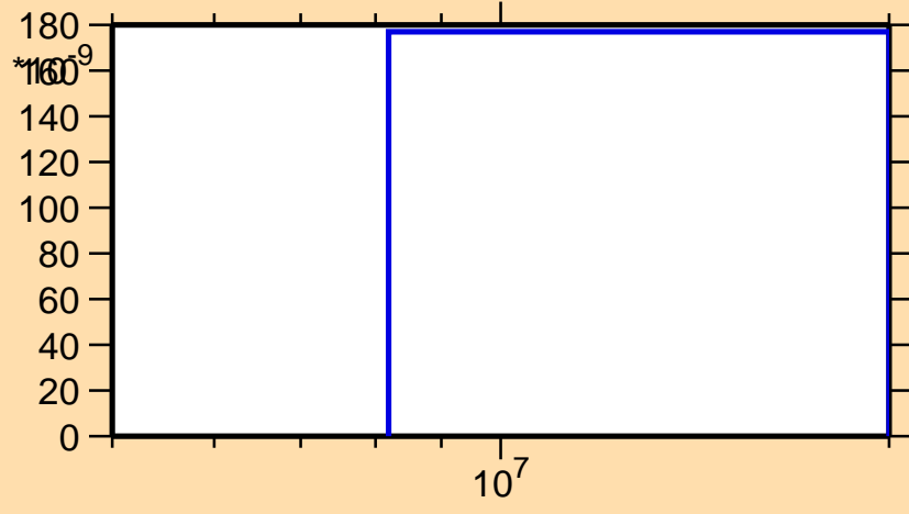
\sigma vs. E for ^{167}\text{W}(n,\text{nd})
