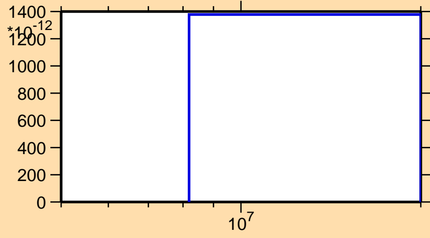
\sigma vs. E for ^{167}\text{W}(\text{mt117})
