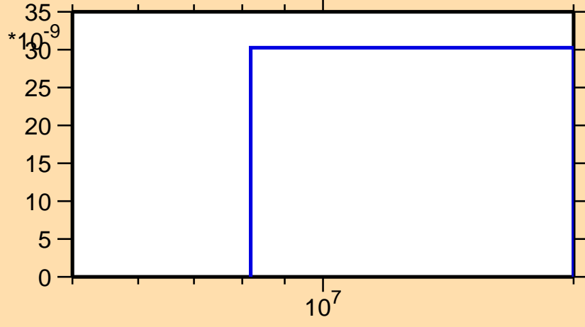
\sigma vs. E for ^{167}\text{W}(n,\text{pt})
