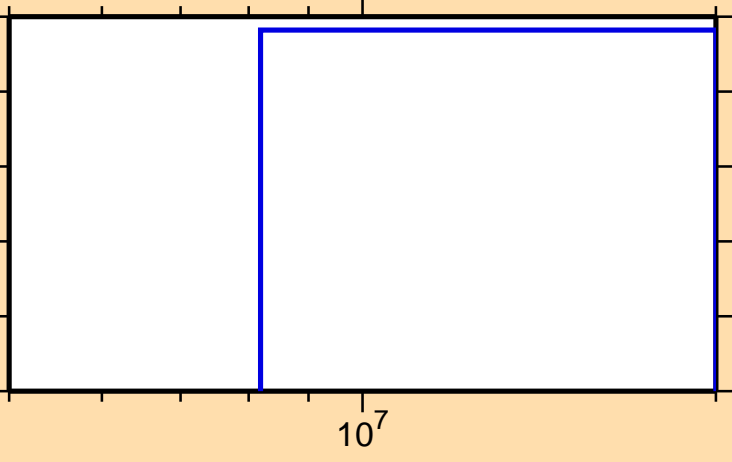
\sigma vs. E for ^{167}\text{W}(n,2n\alpha)
