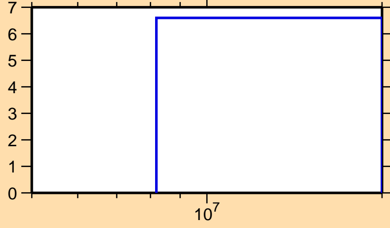
\Delta\sigma/\sigma vs. E for ^{167}\text{W}(n,\text{tot.})
