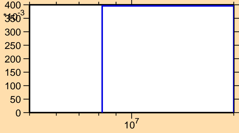
\sigma vs. E for ^{167}\text{W}(n,2n)
