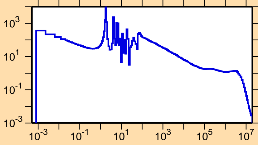
\sigma vs. E for ^{168}\text{W}(n,\gamma)
