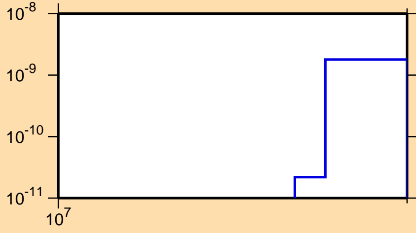
\sigma vs. E for ^{168}\text{W}(n,pt)
