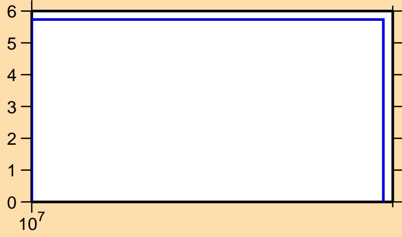
\Delta\sigma/\sigma vs. E for ^{168}\text{W}(n,\text{tot.})
