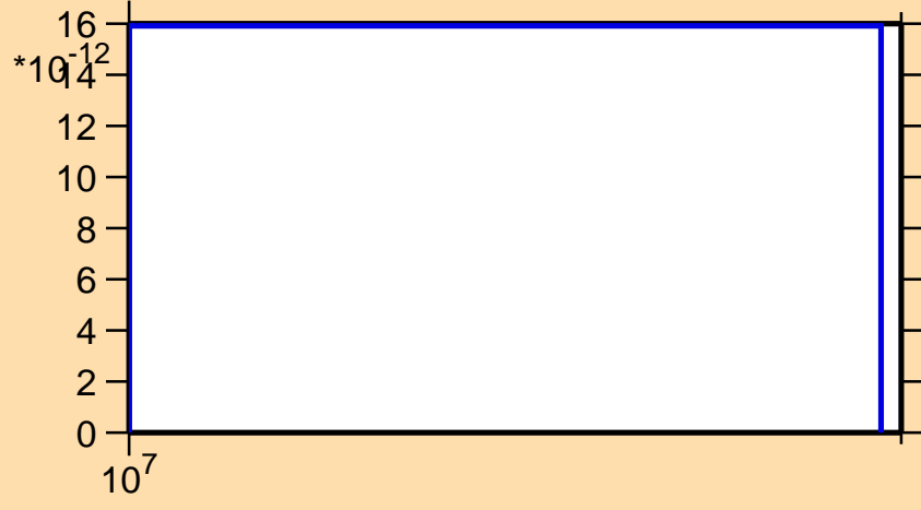
\sigma vs. E for ^{168}\text{W}(n,\text{pt})
