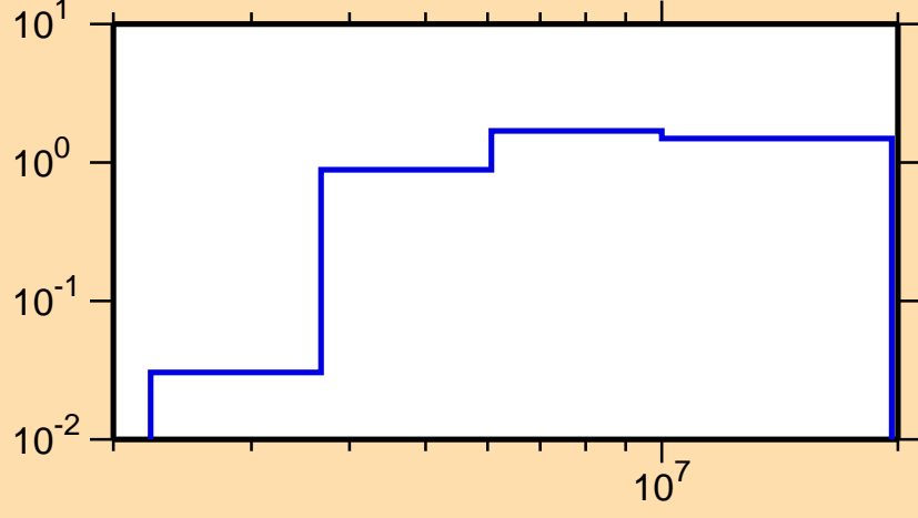
\sigma vs. E for ^{168}\text{W}(n,n\text{cont.})
