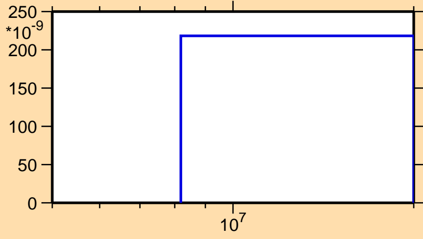
\sigma vs. E for ^{168}\text{W} (mt 45)
