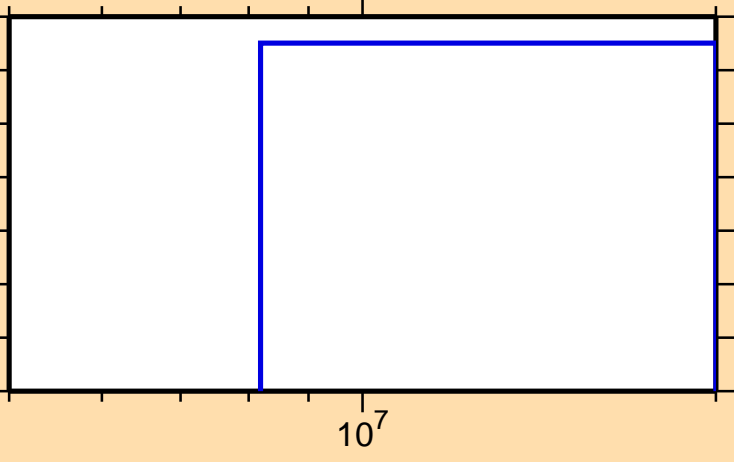
\sigma vs. E for ^{168}\text{W}(n,\text{nd})
