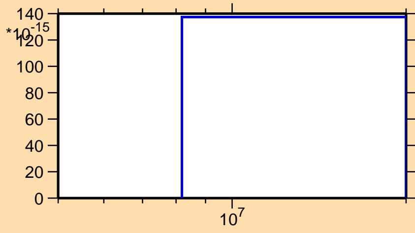
\sigma vs. E for ^{168}\text{W}(n,nt)
