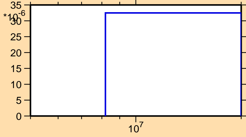
\sigma vs. E for ^{168}\text{W}(n,t)
