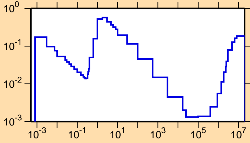
\sigma vs. E for ^{168}\text{W}(n,p)
