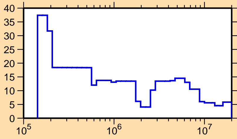
\Delta\sigma/\sigma vs. E for ^{169}\text{W}(n, tot.)
