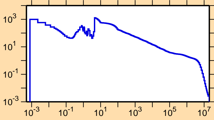
\sigma vs. E for ^{169}\text{W}(n,\gamma)
