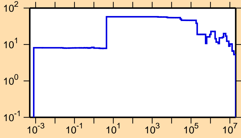
\Delta\sigma/\sigma vs. E for ^{169}\text{W}(n,el.)
