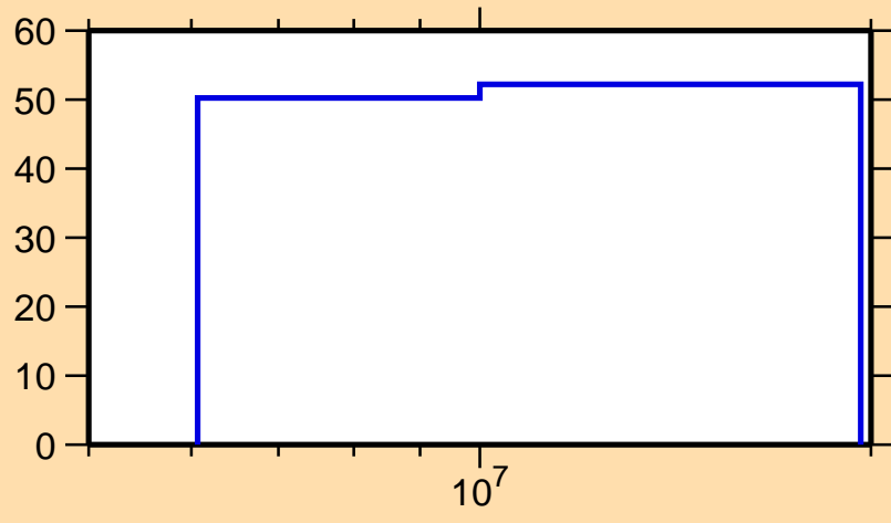
\Delta\sigma/\sigma vs. E for ^{169}\text{W}(n,2n)
