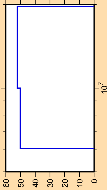
\Delta\sigma/\sigma vs. E for ^{169}\text{W}(n,2n)
