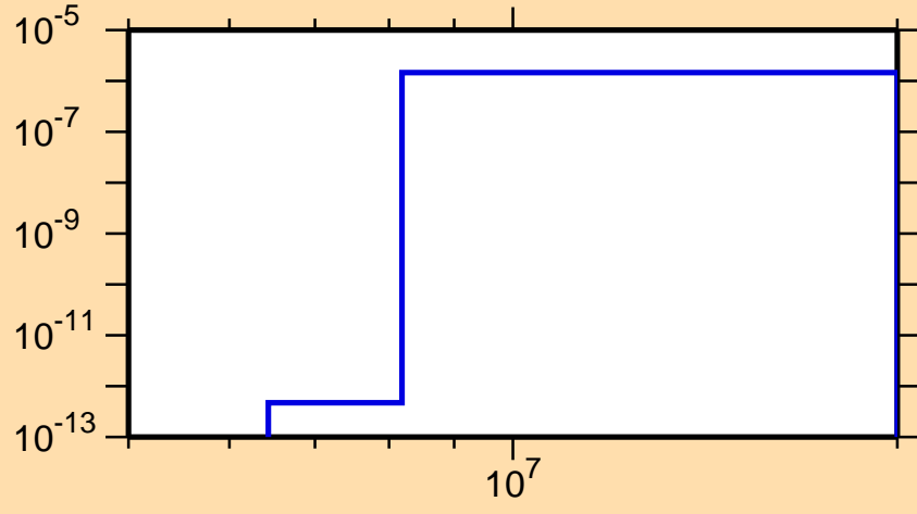
\sigma vs. E for ^{169}\text{W}(n,\text{He3})
