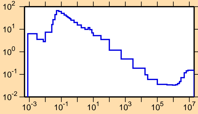
\sigma vs. E for ^{169}\text{W}(n,p)
