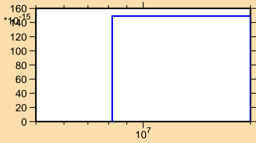
\sigma vs. E for ^{169}\text{W}(n,nt)
