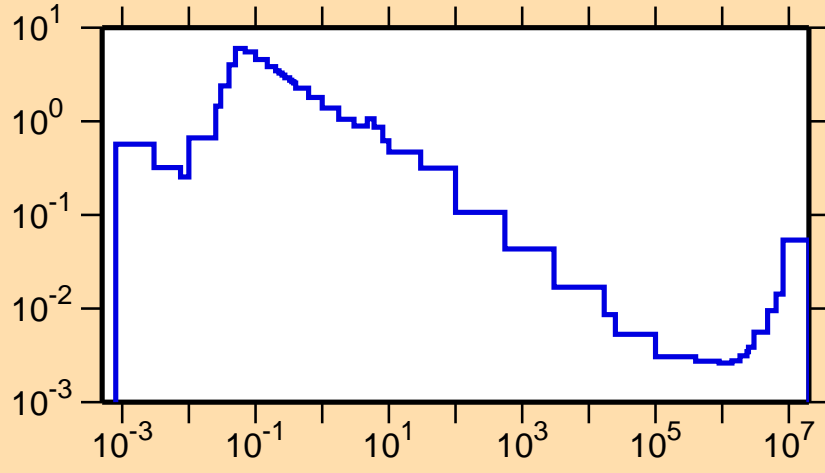
\sigma vs. E for ^{169}\text{W}(n,\alpha)
