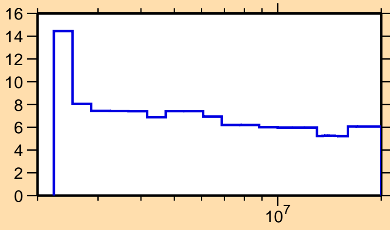
\Delta\sigma/\sigma vs. E for ^{170}\text{W}(n,n\text{oncl.})
