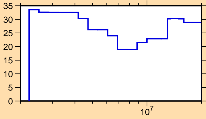
\Delta\sigma/\sigma vs. E for ^{170}\text{W}(n,n\text{cont.})
