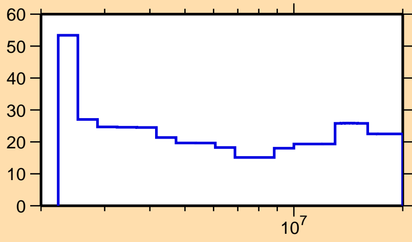
\Delta\sigma/\sigma vs. E for ^{170}\text{W}(n,incl.)
