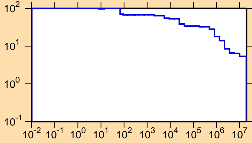
\Delta\sigma/\sigma vs. E for ^{170}\text{W}(n,\text{nonel.})
