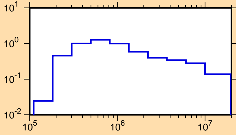
\sigma vs. E for ^{170}\text{W}(n,n_1)
