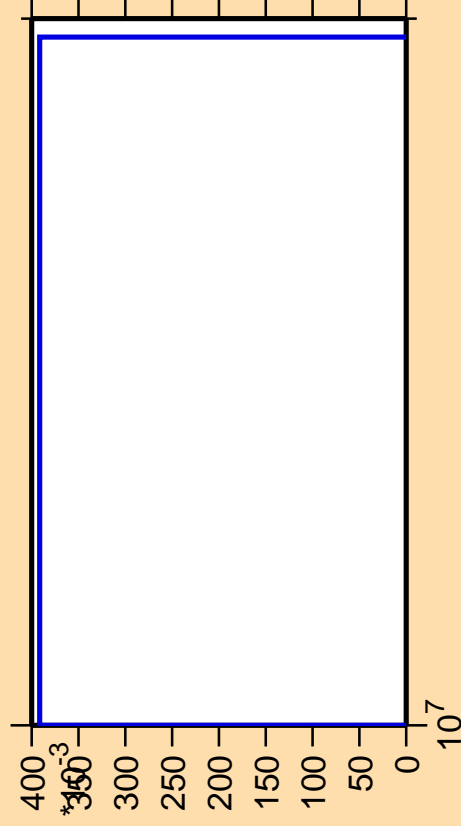
\Delta\sigma/\sigma vs. E for ^{170}\text{W} (mt 34)
