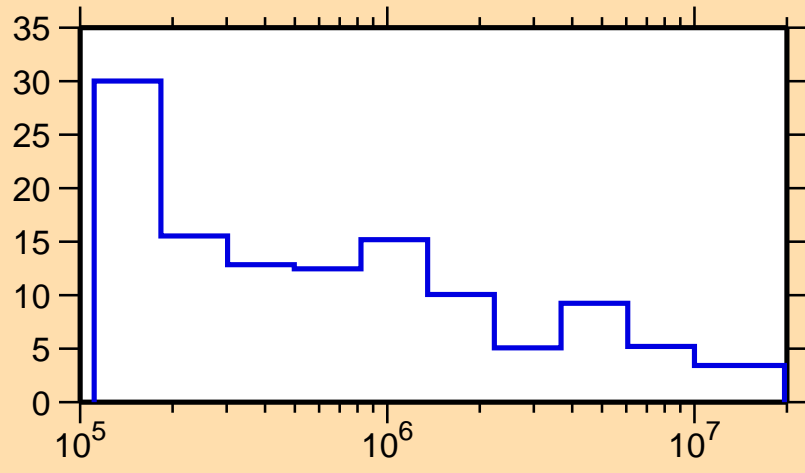
\Delta\sigma/\sigma vs. E for ^{170}\text{W}(n,\text{tot.})
