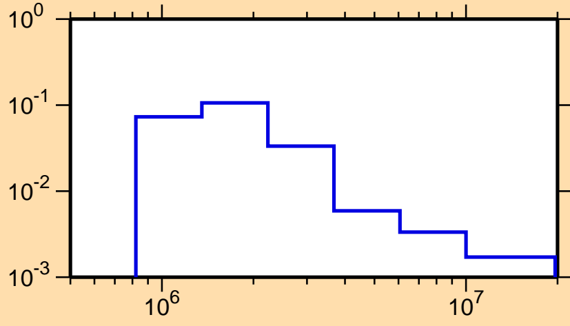
\sigma vs. E for ^{170}\text{W}(n,n_4)
