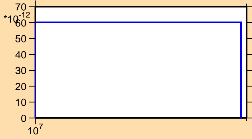
\sigma vs. E for ^{170}\text{W}(\text{mt117})
