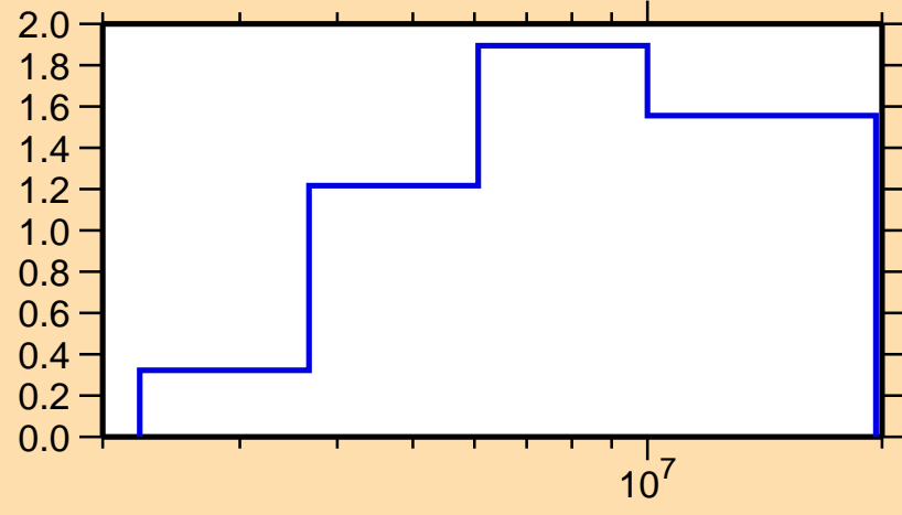
\sigma vs. E for ^{170}\text{W}(n,n\text{cont.})
