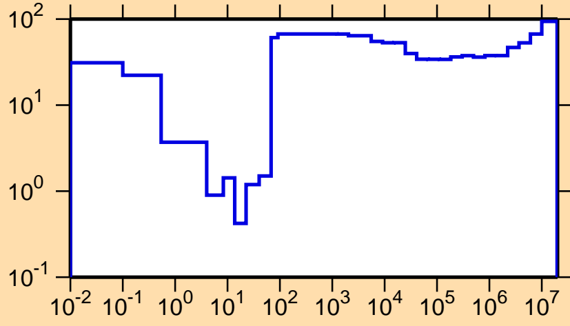
\Delta\sigma/\sigma vs. E for ^{170}\text{W}(n,\gamma)
