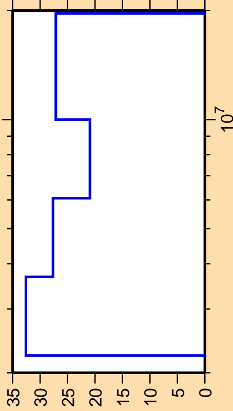
\Delta\sigma/\sigma vs. E for ^{170}\text{W}(n,n\text{cont.})
