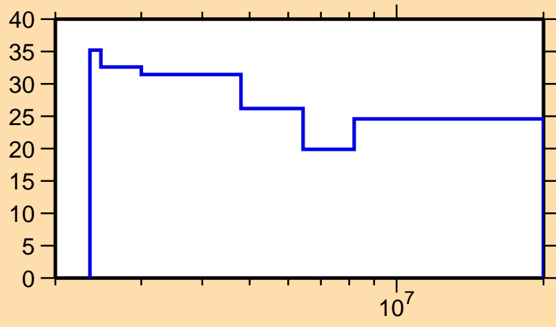
\Delta\sigma/\sigma vs. E for ^{170}\text{W}(n,n\text{cont.})
