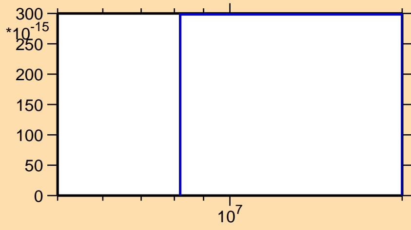
\sigma vs. E for ^{170}\text{W}(n,nt)
