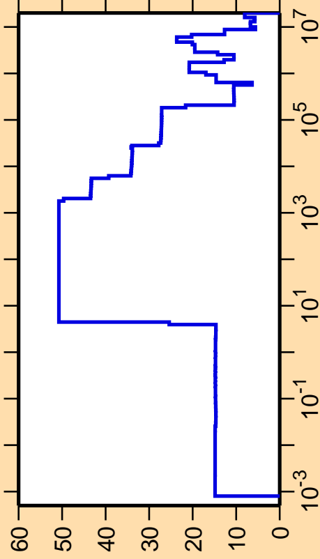
\Delta\sigma/\sigma vs. E for ^{171}\text{W}(n,\text{el.})
