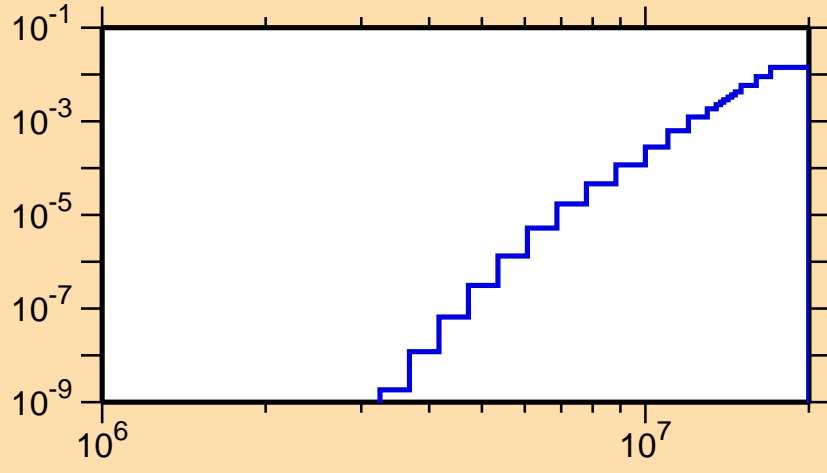
\sigma vs. E for ^{171}\text{W}(n,n\alpha)
