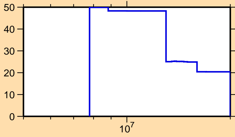
\Delta\sigma/\sigma vs. E for ^{171}\text{W}(n,2n)
