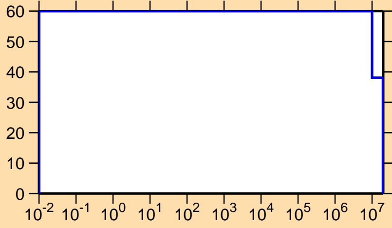
\Delta\sigma/\sigma vs. E for ^{171}\text{W}(n,p)
