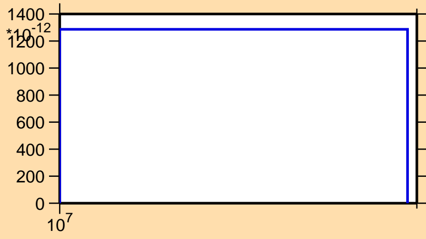
\sigma vs. E for ^{171}\text{W} (mt 45)
