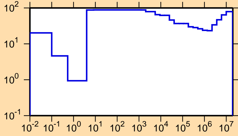
\Delta\sigma/\sigma vs. E for ^{171}\text{W}(n,\gamma)
