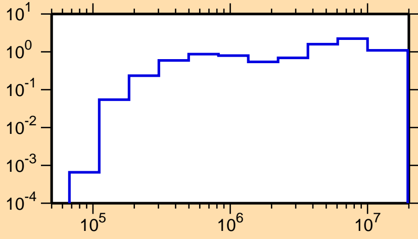
\sigma vs. E for ^{171}\text{W}(n,\text{inel.})
