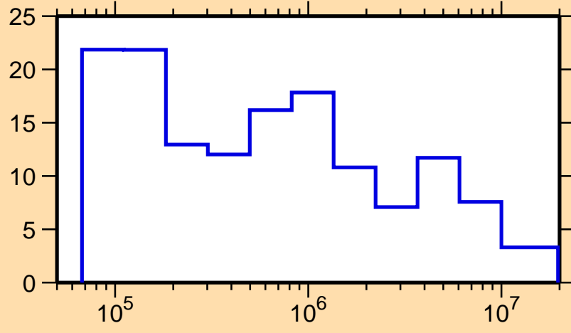
\Delta\sigma/\sigma vs. E for ^{171}\text{W}(n,\text{tot.})
