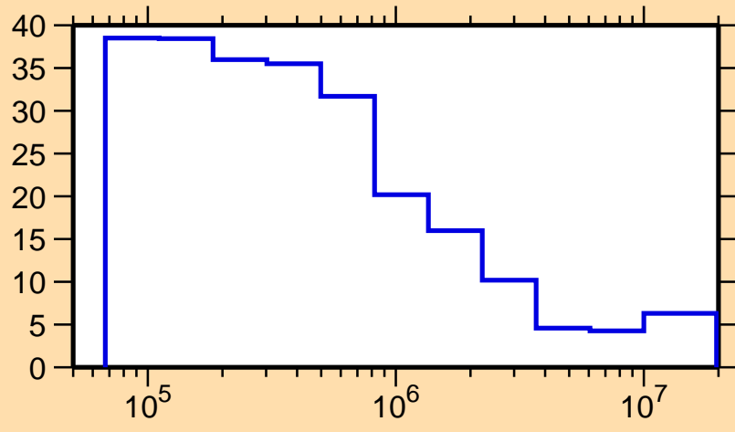
\Delta\sigma/\sigma vs. E for ^{171}\text{W}(n,\text{nonel.})
