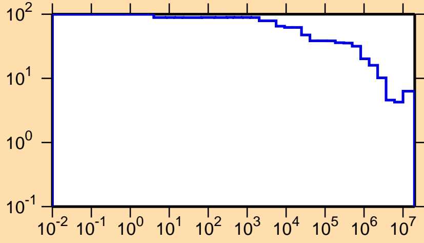
\Delta\sigma/\sigma vs. E for ^{171}\text{W}(n,\text{nonel.})
