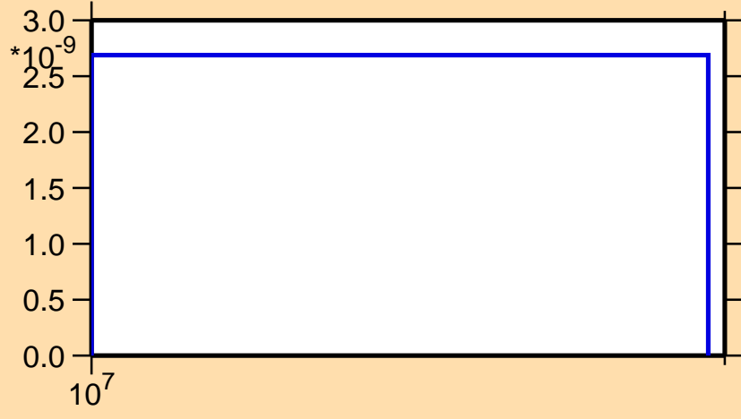
\sigma vs. E for ^{171}\text{W}(n,\text{pd})
