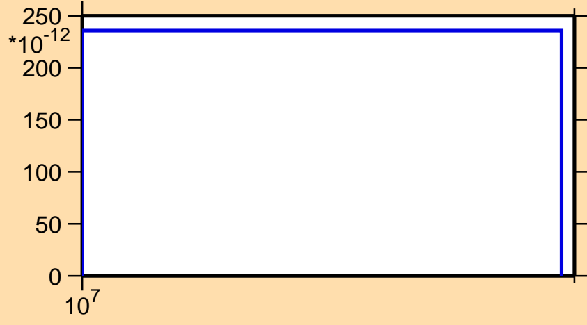
\sigma vs. E for ^{171}\text{W}(n,\text{pt})
