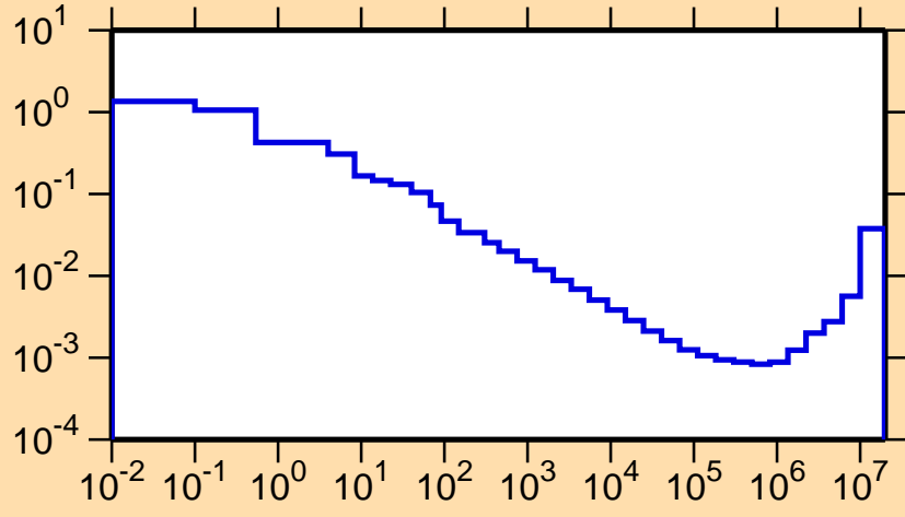
\sigma vs. E for ^{171}\text{W}(n,\alpha)
