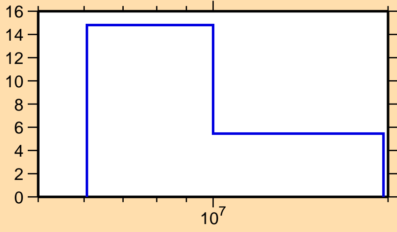
\Delta\sigma/\sigma vs. E for ^{171}\text{W}(n,\text{el.})
