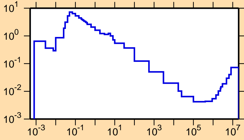
\sigma vs. E for ^{171}\text{W}(n,p)
