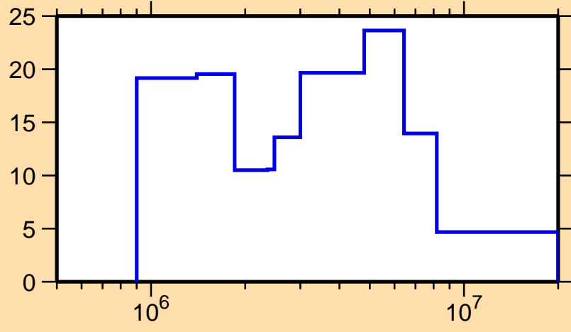
\Delta\sigma/\sigma vs. E for ^{171}\text{W}(n, el.)
