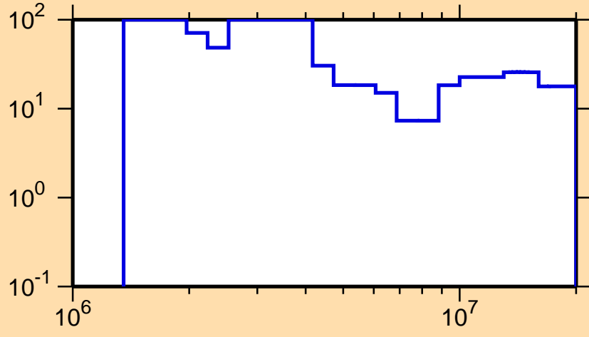
\Delta\sigma/\sigma vs. E for ^{172}\text{W}(n,n\text{cont.})
