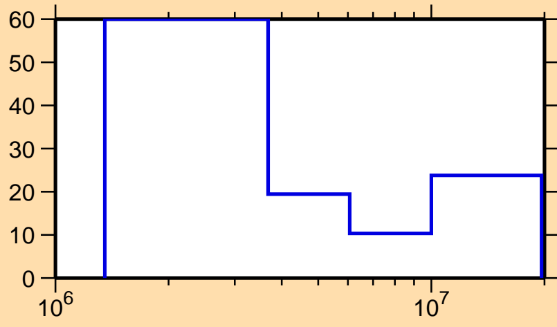
\Delta\sigma/\sigma vs. E for ^{172}\text{W}(n,n\text{cont.})
