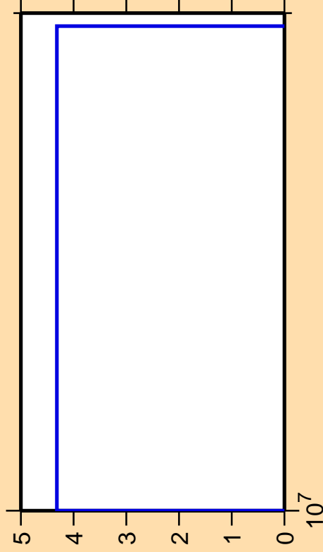
\Delta\sigma/\sigma vs. E for ^{172}\text{W}(n,nt)
