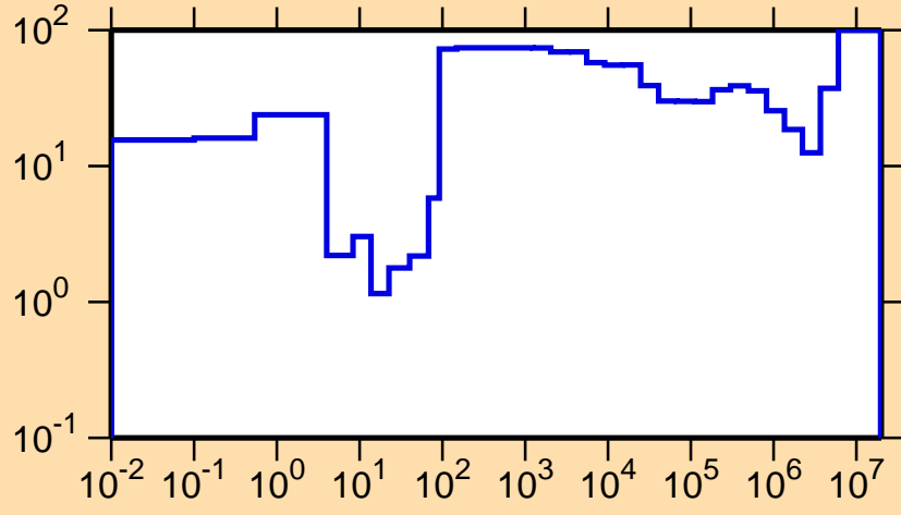
\Delta\sigma/\sigma vs. E for ^{172}\text{W}(n,\gamma)
