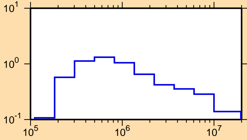
\sigma vs. E for ^{172}\text{W}(n,n_1)
