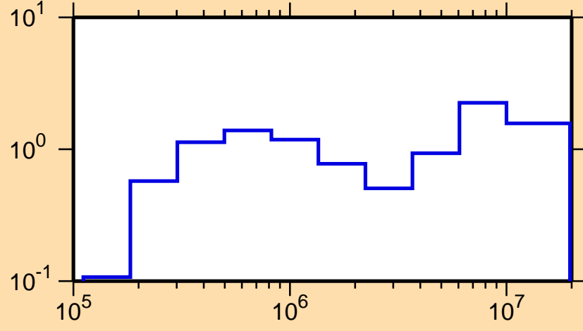
\sigma vs. E for ^{172}\text{W}(n,\text{inel.})
