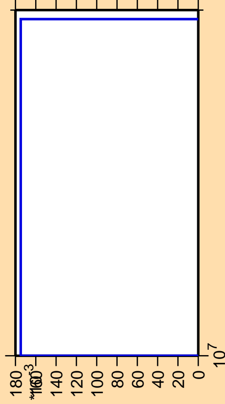
\Delta\sigma/\sigma vs. E for ^{172}\text{W} (mt 34)
