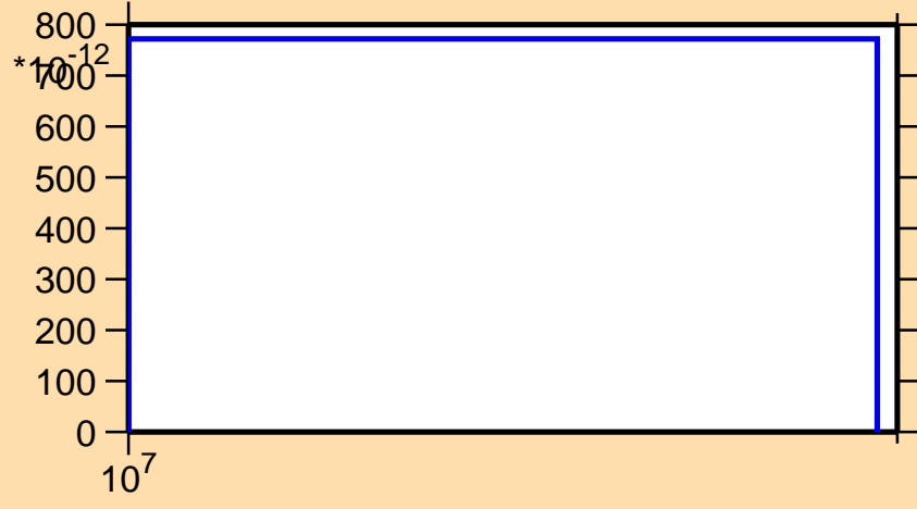
\sigma vs. E for ^{172}\text{W}(n,\text{pd})
