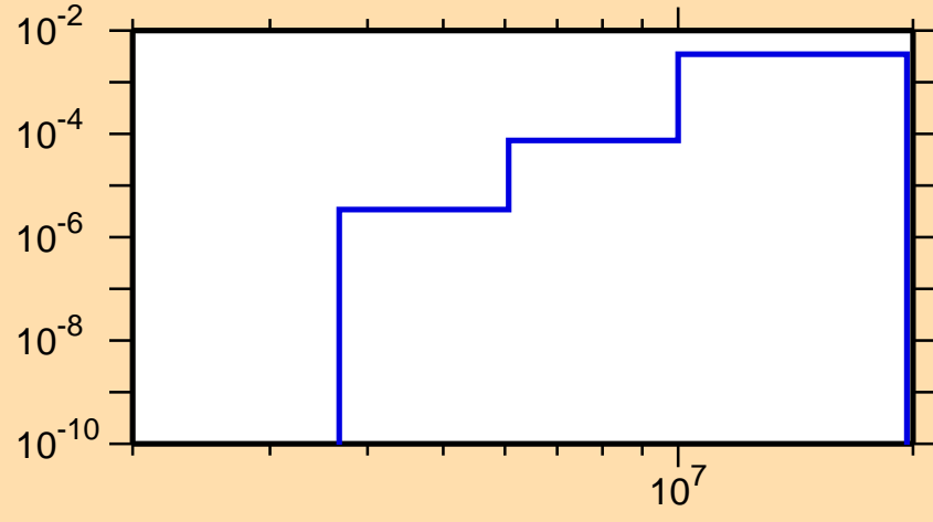
\sigma vs. E for ^{172}\text{W}(n,n\alpha)
