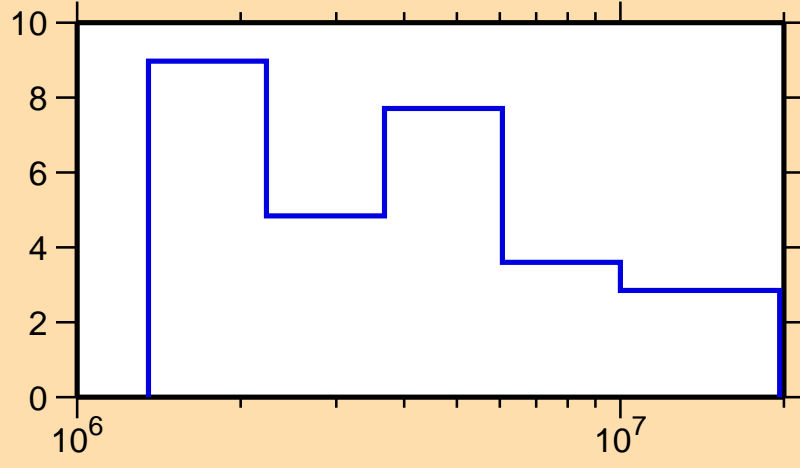
\Delta\sigma/\sigma vs. E for ^{172}\text{W}(n,\text{tot.})
