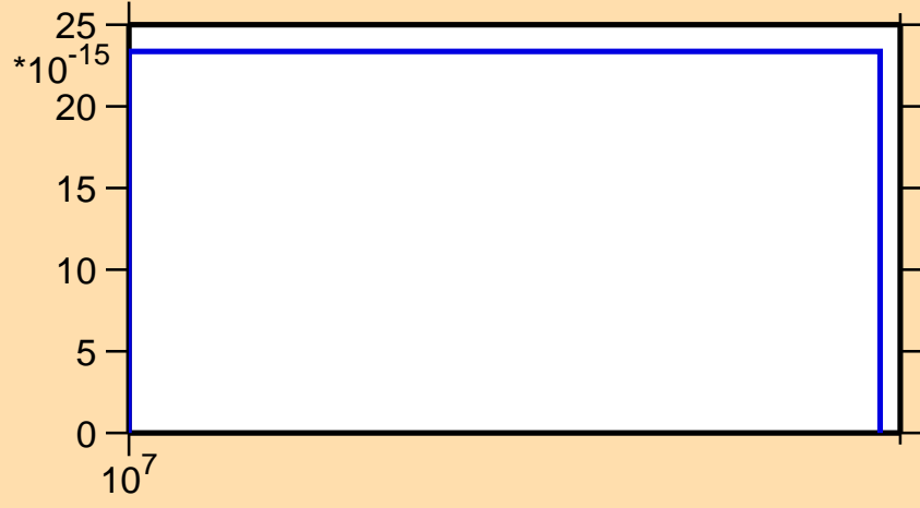
\sigma vs. E for ^{172}\text{W} (mt 34)
