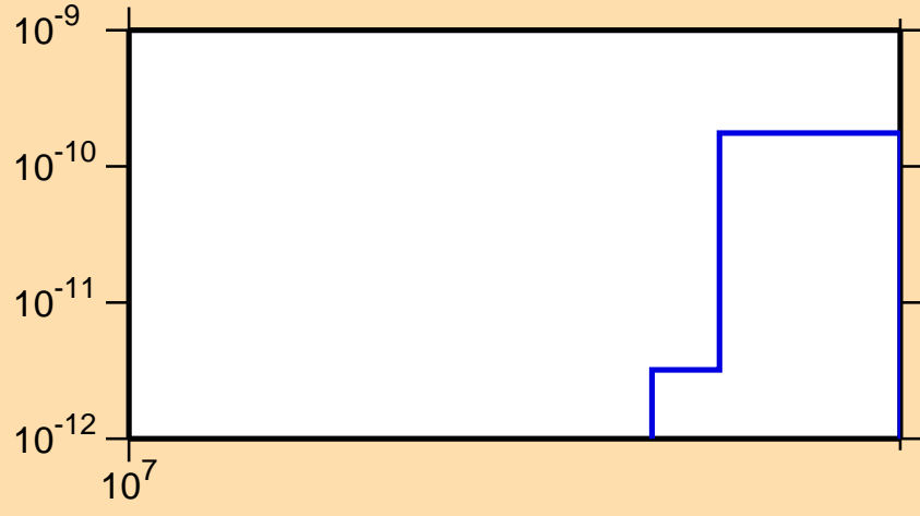
\sigma vs. E for ^{173}\text{W} (mt 34)
