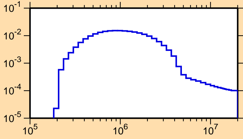
\sigma vs. E for ^{173}\text{W}(n,n_4)
