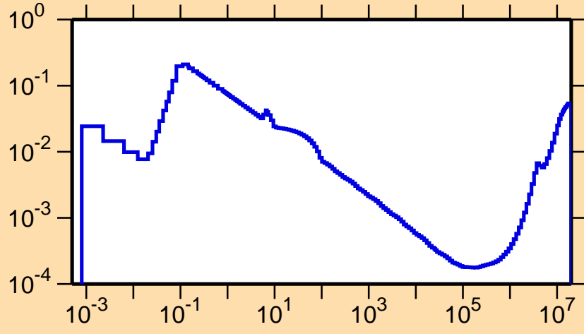
\sigma vs. E for ^{173}\text{W}(n,p)
