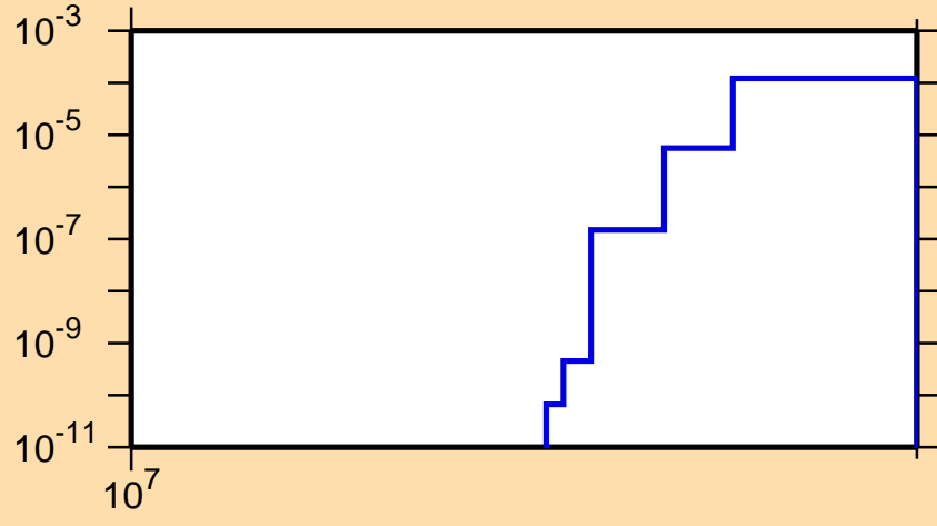
\sigma vs. E for ^{173}\text{W}(n,2np)
