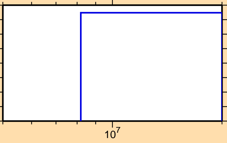
\sigma vs. E for ^{173}\text{W}(n,\text{pt})
