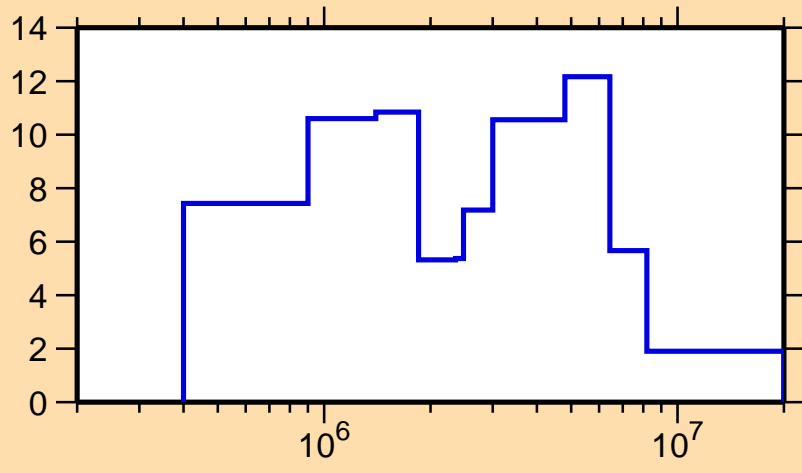
\Delta\sigma/\sigma vs. E for ^{173}\text{W}(n,el.)
