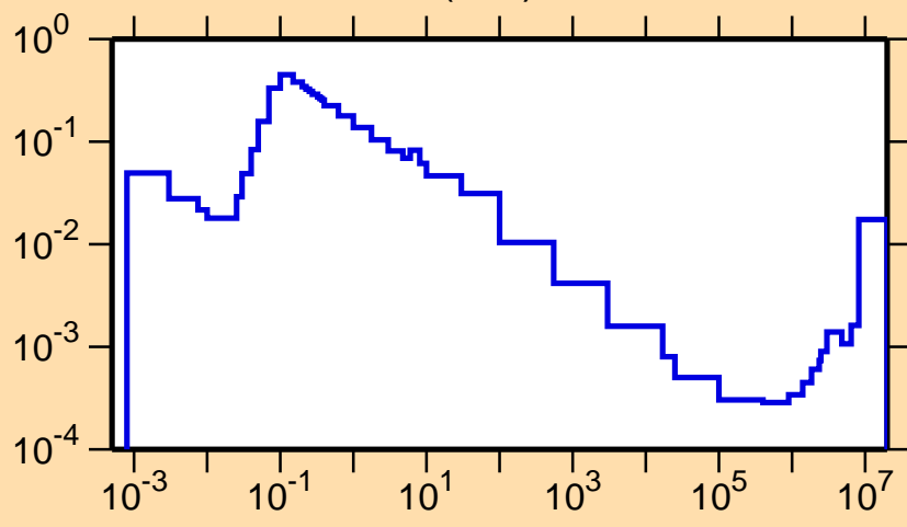
\sigma vs. E for ^{173}\text{W}(n,\alpha)
